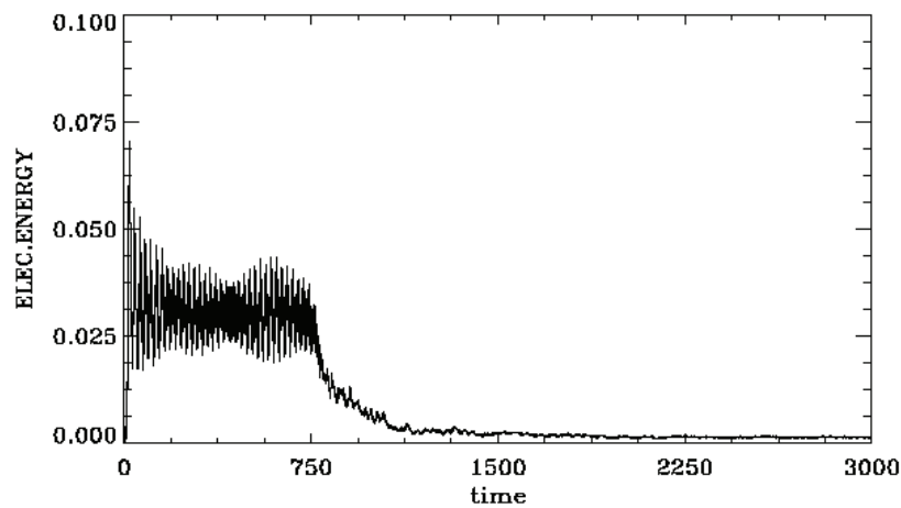
Fig. 1. Time evolution of the electric field energy
