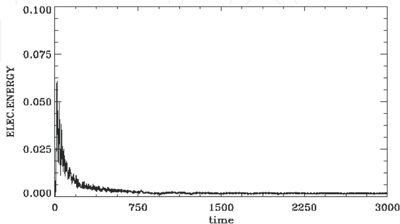
Fig. 25. Time evolution of the electric field energy.
