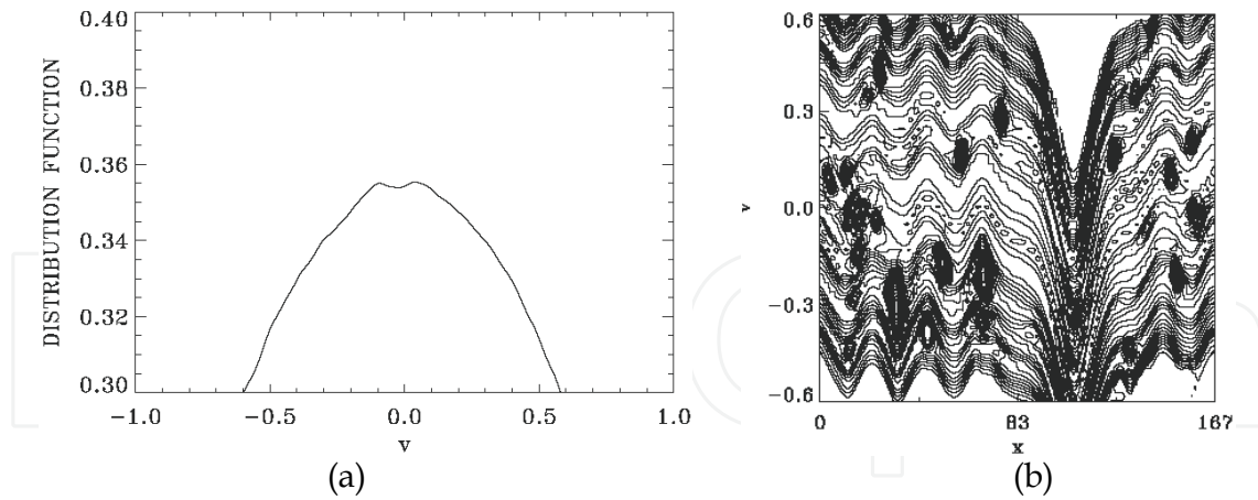
Fig. 30. (a) Same as Fig.(29a) (concentrates on the top) (b) Contour plot for the distribution in Fig.(30a)
