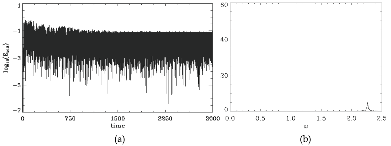
Fig. 42. (a) Time evolution of the Fourier mode k=0.45 , (b) Spectrum of the Fourier mode k=0.45
