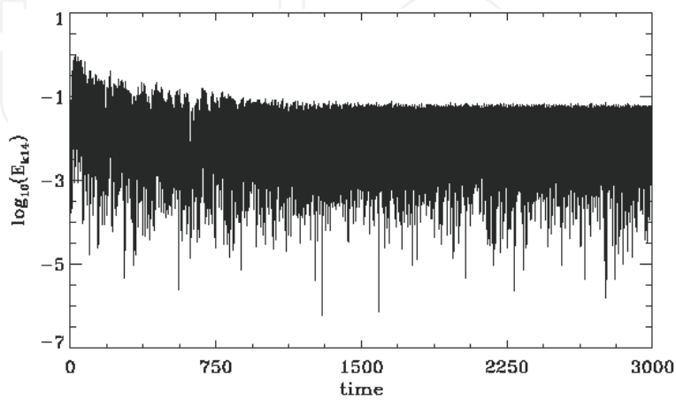
Fig. 43. Time evolution of the Fourier mode k=0.525
