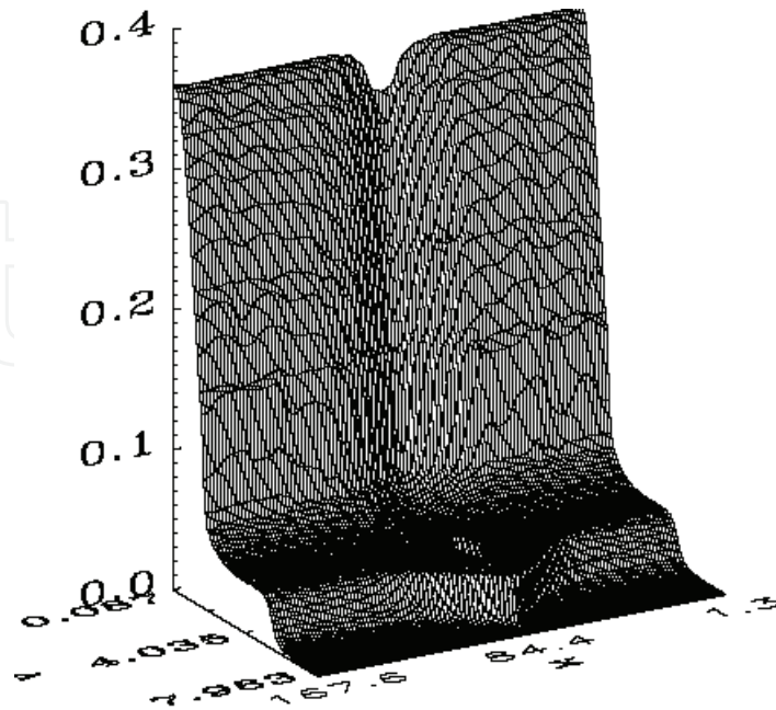
Fig. 8. Three-dimensional view of the results in Fig.7o.
