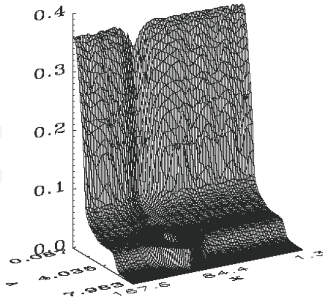
Fig. 28. Same as Fig.(27o), 3D plot at t = 3000
