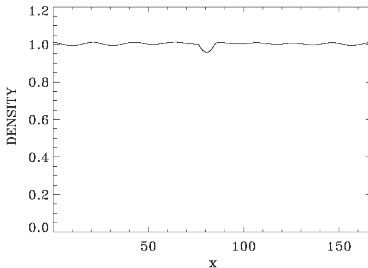
Fig. 24. Electron density profile at t=2980 .
