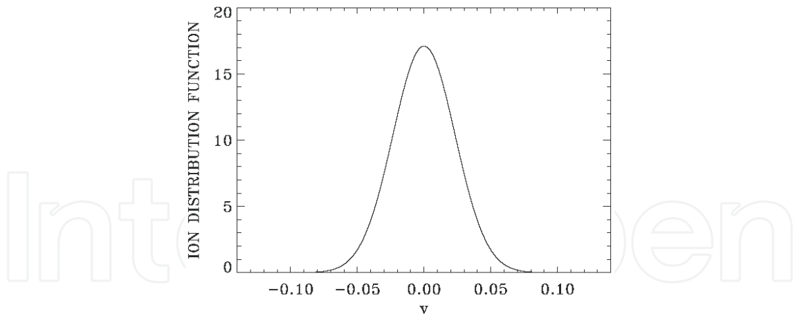
Fig. 10. Ion distribution function at t = 2980
