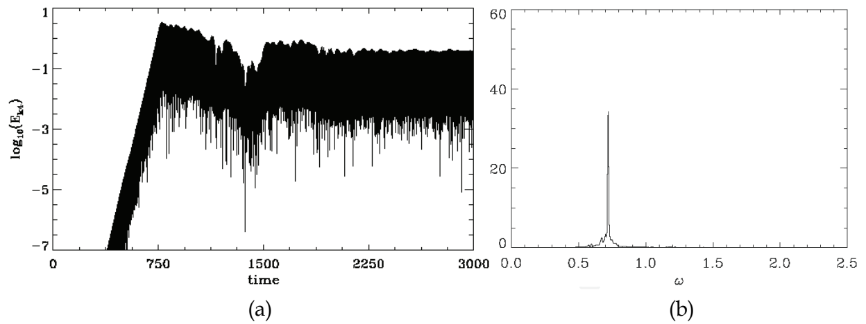
Fig. 15. (a) Time evolution of the Fourier mode with k=0.15 (b) Spectrum of the Fourier mode k=0.15
