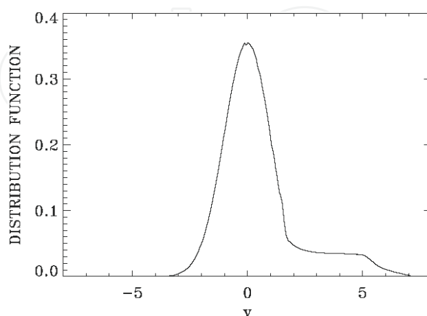
Fig. 9. Electron distribution function at t = 2980 .
