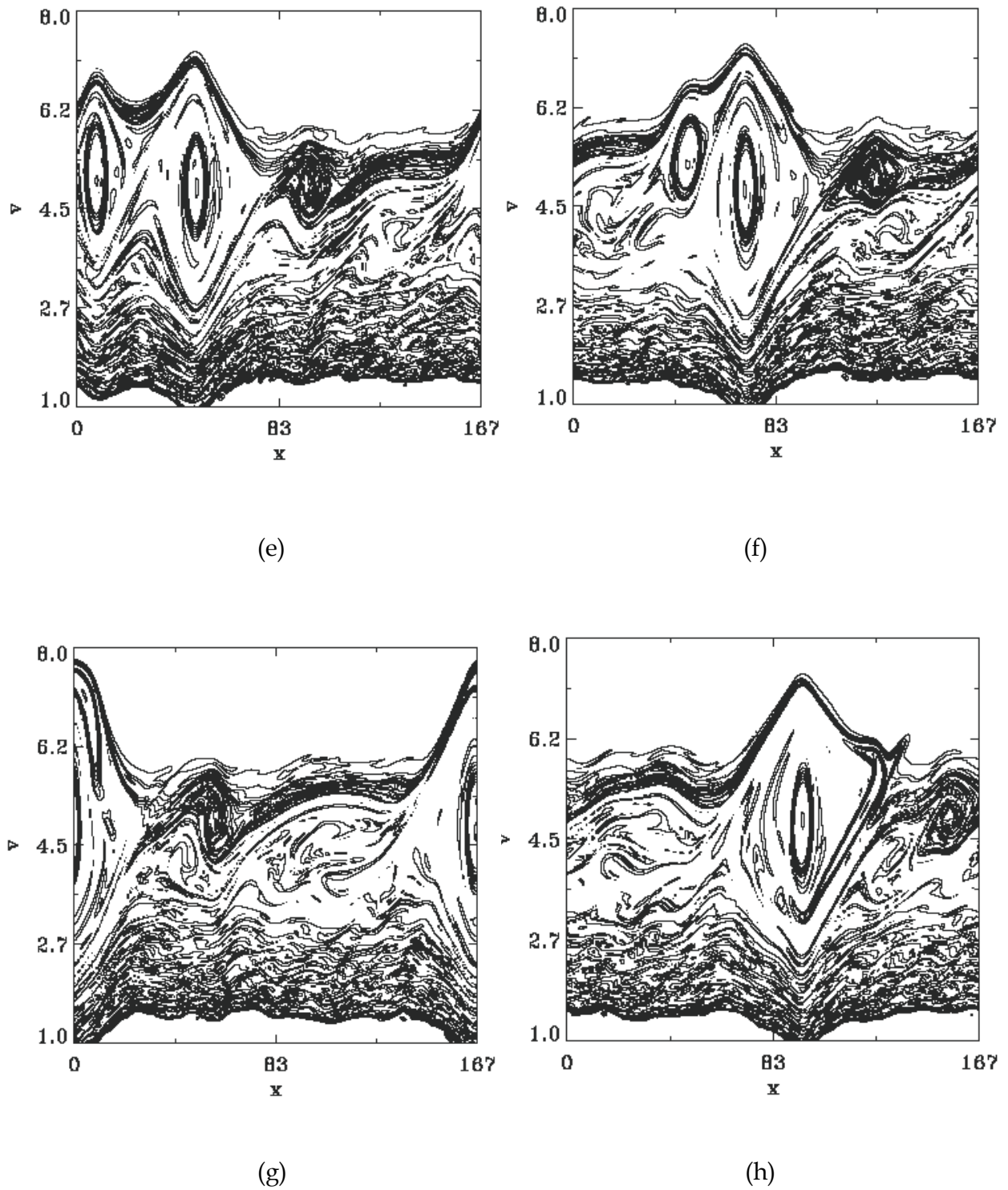
Fig. 27. (e) Contour plot of the distribution function, t = 720 (f) Contour plot of the distribution function, t = 760 (g) Contour plot of the distribution function, t = 780 (h) Contour plot of the distribution function, t = 800
