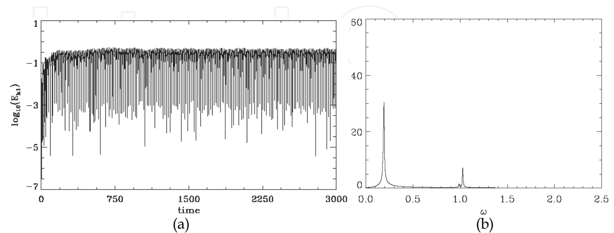
Fig. 32. (a) Time evolution of the Fourier mode k=0.0375 , (b) Spectrum of the Fourier mode k=0.0375
