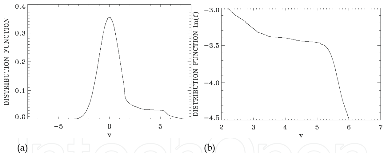
Fig. 29. (a) Spatially averaged distribution function, t = 3000 (b) Same as Fig.(29a), concentrating on the tail region.
