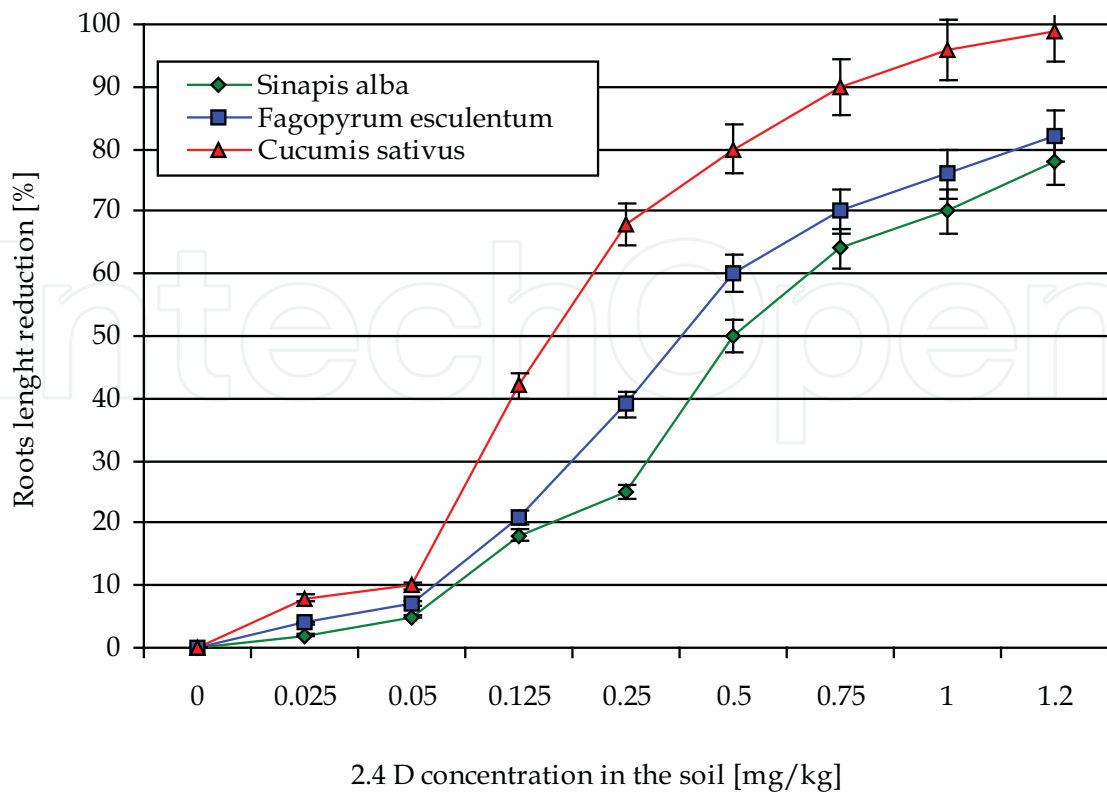
Fig. 1. 2,4 D effect on the tested plant in terms of roots length reduction
