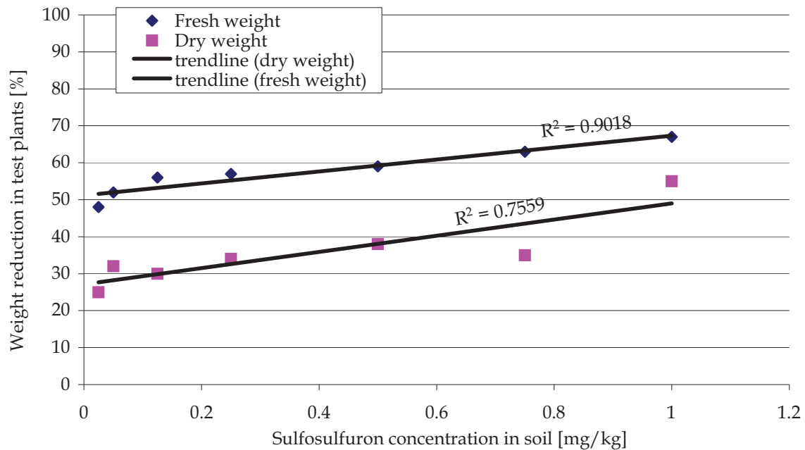
Fig. 4. Changes fresh and dry weight of Sinapis alba under the influence of different sulfosulfuron concentrations in soil
