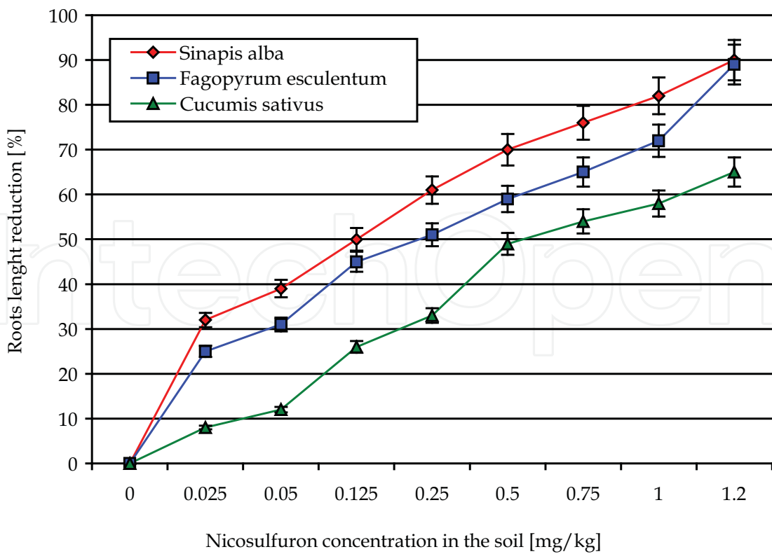
Fig. 2. Nicosulfuron effect on the tested plant in terms of roots length reduction
