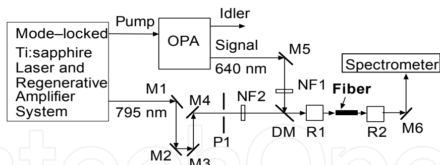
Fig. 10. Layout of the experimental setup. (Xu et al., 1999) M, silver-coated plane mirrors; R1 and R2, reflective objectives (36 \times ); DM, dichroic mirror; NF1 and NF2, valuable optical attenuators; OPA, optical parametric amplifier.
