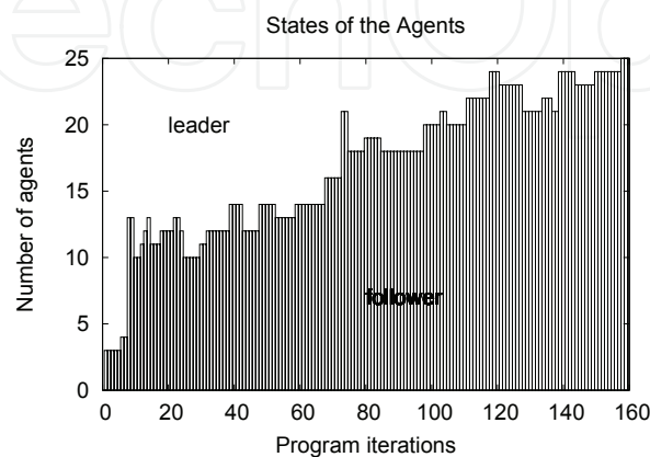
Fig. 7. States of flocking robots during the experiment illustrated in Figure 6 (León-Fernández & Muñoz-Meléndez, 2007).
