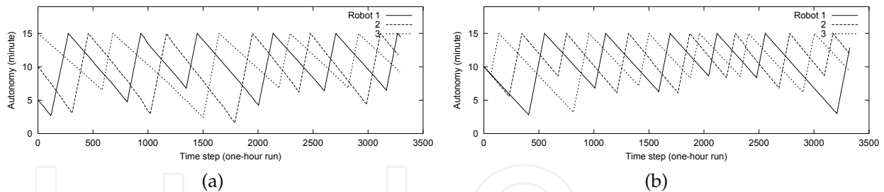
Fig. 1. Autonomy of three mobile robots sharing a charging station using a basic strategy with a 7.5-minute recharge threshold (a), and using an opportunistic strategy with a flexible recharge threshold (b) (Sempé et al., 2002).
