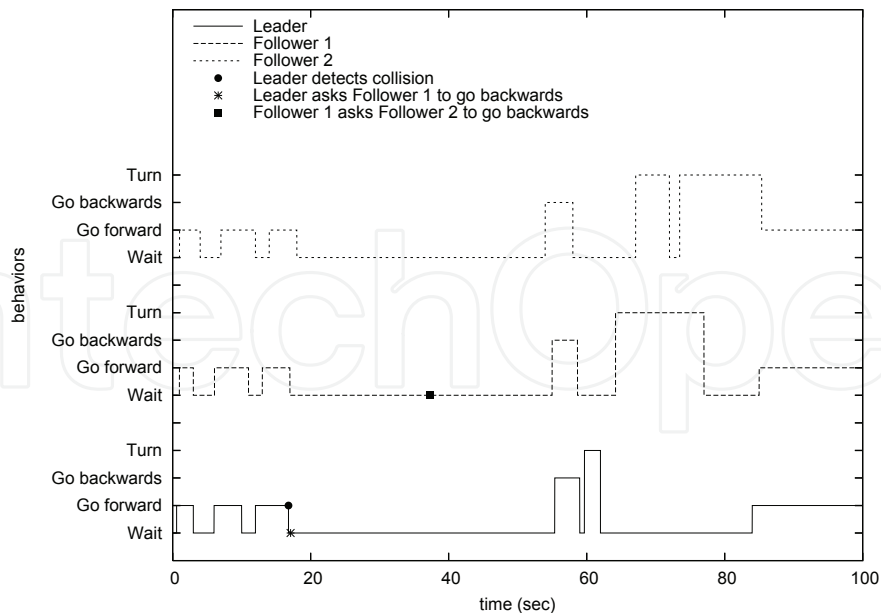
Fig. 5. Behaviors executed and time in which robots of the Mini-trans system send messages during the experiment illustrated in Figure 4 (Jiménez-Velasco & Muñoz-Meléndez, 2006).
