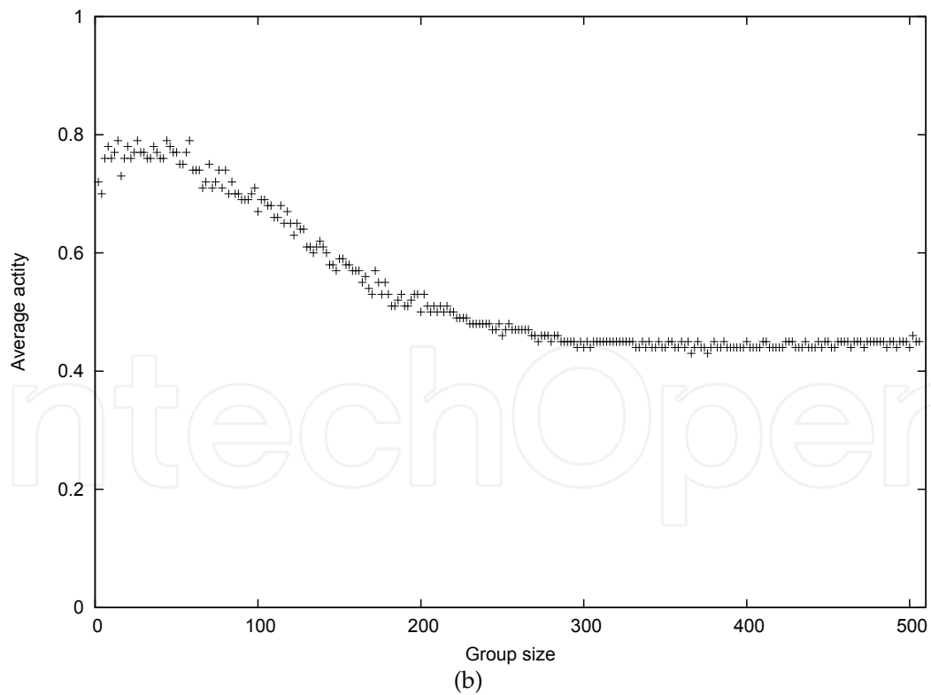
Fig. 8. Average speed (a) and average activity (b) of a foraging multi-robot system under different conditions of group size. The average speed is given in units of the simulation environment, where 1 unit is around 1m. The activity is a value between 0 and 1. All the experiments lasted 350 iterations of the program.
