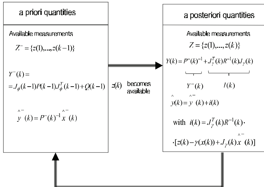
Fig. 6. Schematic diagram of the Extended Information Filter loop
