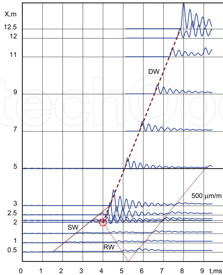
Fig. 14. X-t diagram of strain wave propagation under radiolysis gas detonation: scale of a strain signal is shown on the right axis (1 division is 500 \mu\text{m}/\text{m} or 0.05\% ): SW = precursor shock wave; DW = detonation wave; RW = retonation wave
