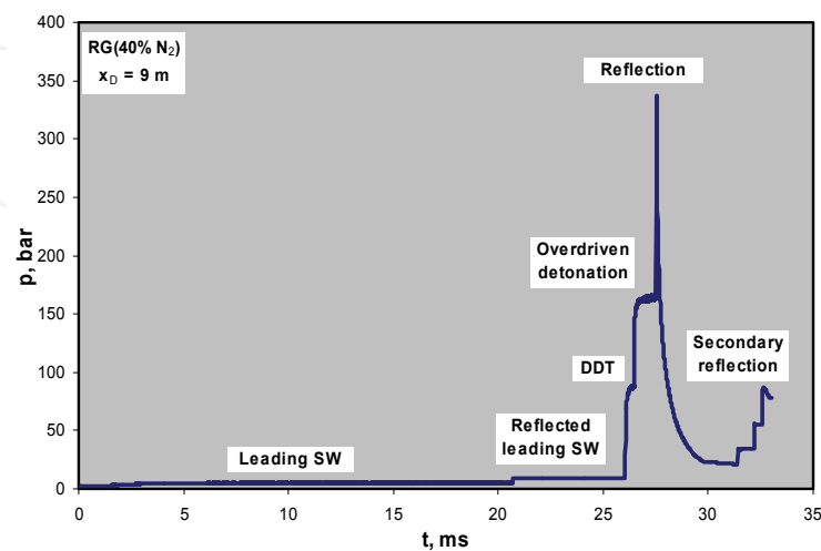
Fig. 17. Computed x - t -diagram (top) and computed peak pressure record (bottom) for radiolysis gas with 40 vol% nitrogen and a DDT point at x_D = 9 m
