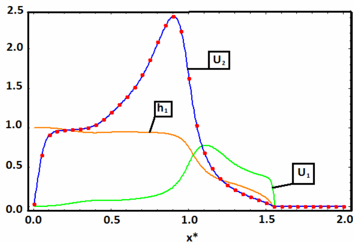
Fig. 11. Dimensionless profiles of the gravity current's thickness and the velocities. Run 9, 5.6 sec after the removal of the lock
