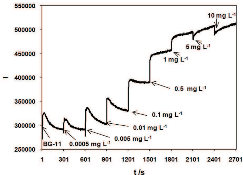
Fig. 1. Fluorescence response of a Dictyosphaerium chlorelloides membrane to simazine increasing concentrations in the range of 5 \times 10^{-4} to 10 \text{ mg L}^{-1} . \lambda_{\text{exc}} : 467 nm, \lambda_{\text{em}} : 699 nm. (From Peña-Vázquez et al., (2010), supplemented material).
