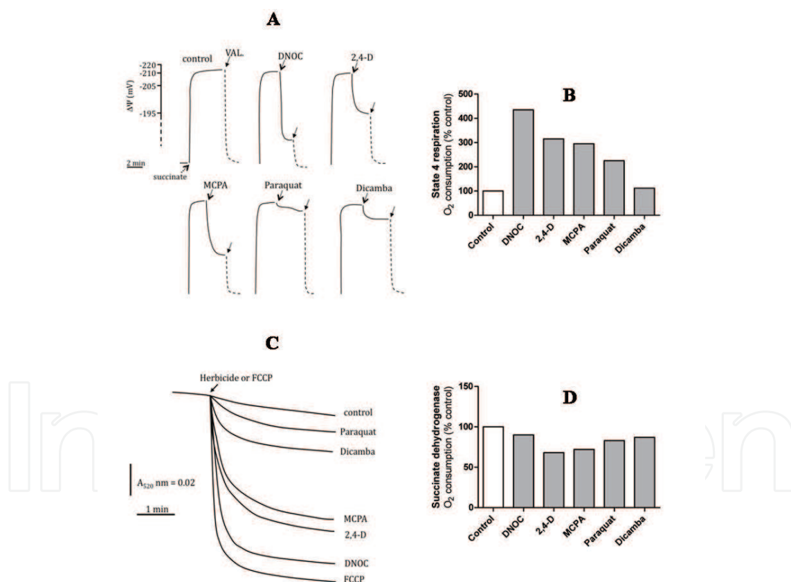
Fig. 1. Effects of DNOC (80 \mu\text{M} ), 2,4-D (3 mM), MCPA (3 mM), paraquat (40 mM) and dicamba (2 mM) on succinate-supported transmembrane potential ( \Delta\Psi ) (A), state 4 \text{O}_2 consumption (B), swelling in hypo-osmotic \text{K}^+ -acetate medium (C), and succinate dehydrogenase activity (D) of potato tuber mitochondria. Val., valinomycin; FCCP, carbonyl cyanide p -trifluoromethoxyphenyl-hydrazone. The traces represent typical recordings from several experiments with different mitochondrial preparations.
