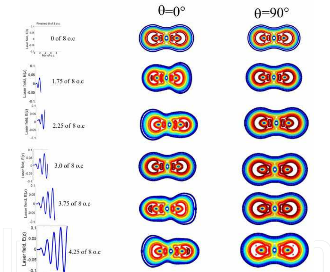
Fig. 3c. Snapshot of the isosurface of the TDELDF images for I_0 = 3.5 \times 10^{14} \text{ W/cm}^2 as the CO 2 molecule evolves in the laser field. Calculations are done for with \theta=0^\circ and \theta=90^\circ .
