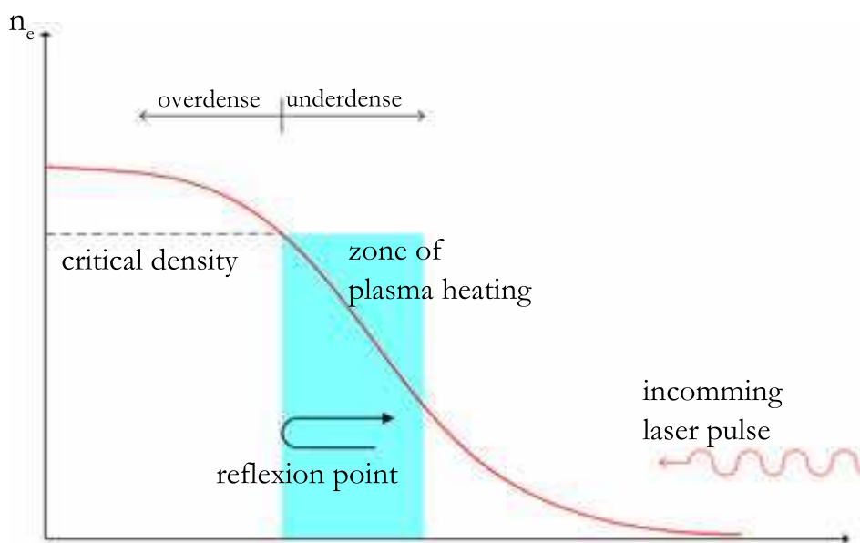
Fig. 1. One-dimensional illustration of the collisional absorption effect.
