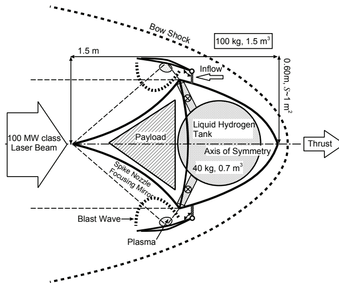
Fig. 1. Air-breathing pulse-laser powered vehicle(Myрабо, 2001).
