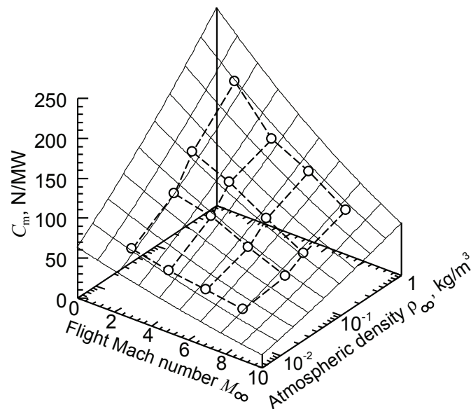
Fig. 9. C_m map of the laser ramjet.
