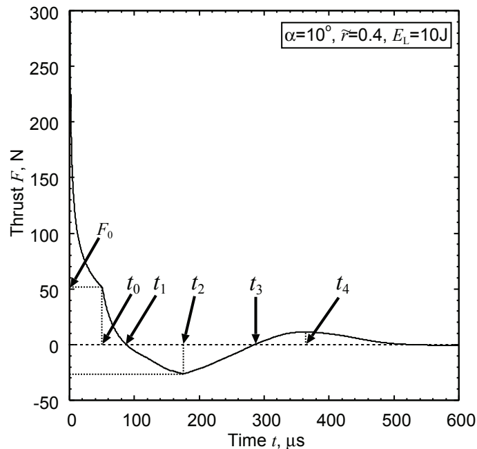
Fig. 5. Thrust history. ( \eta_{bw}=0.43 )
