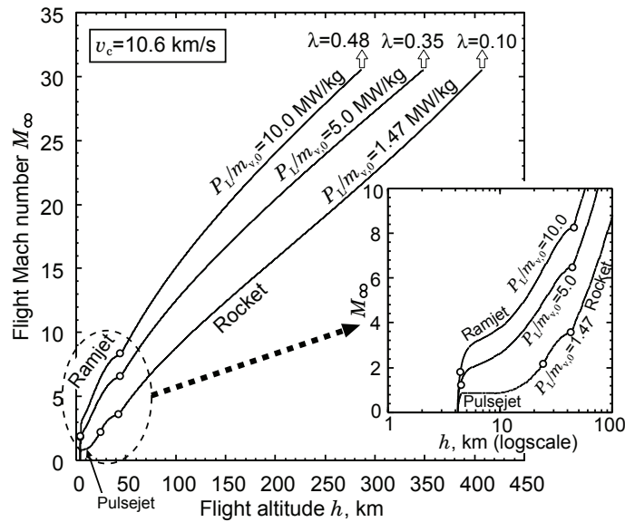
Fig. 13. Flight Mach number vs. flight altitude.
