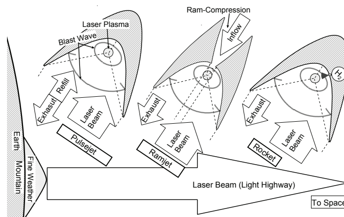
Fig. 2. A pulse-laser powered orbital launching system.
