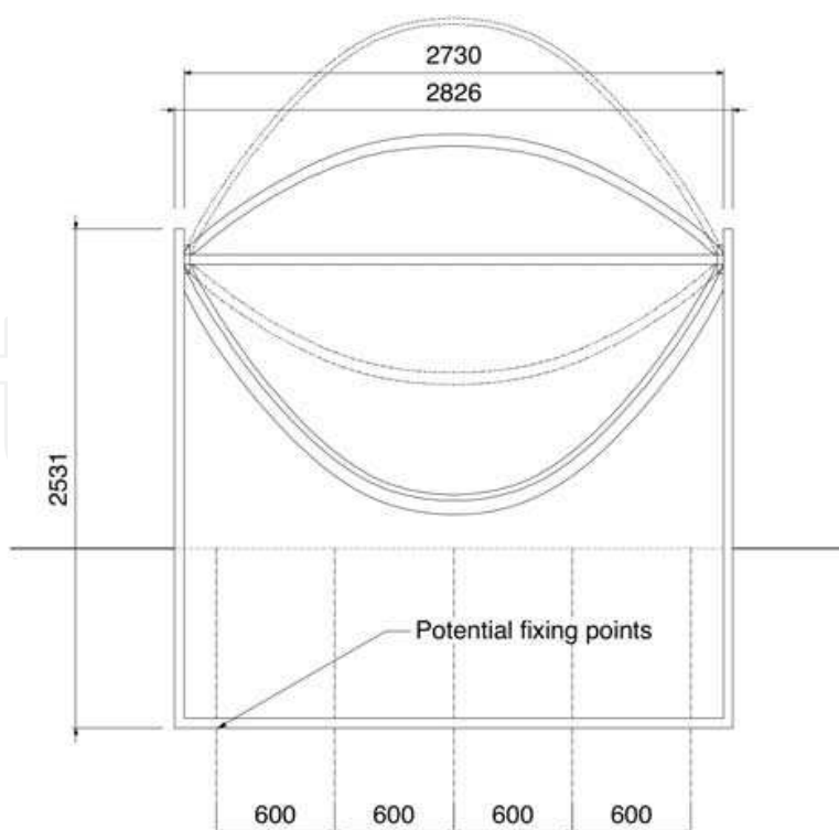
Fig. 9. Overall dimensions and fixing points
