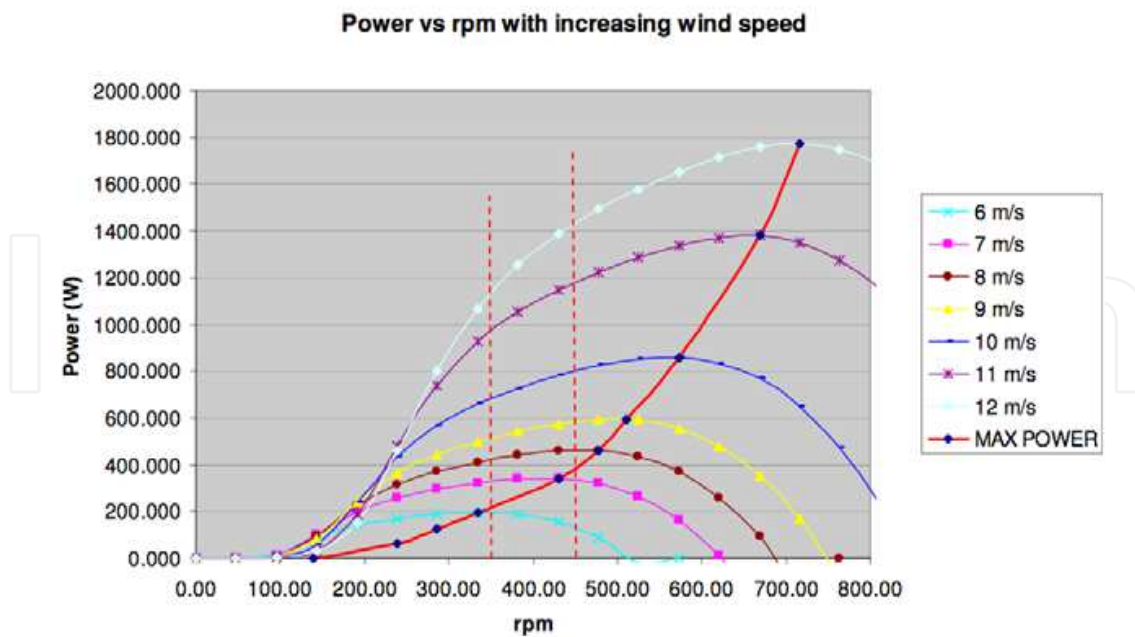
Fig. 8. Power vs rpm with increasing wind speed
