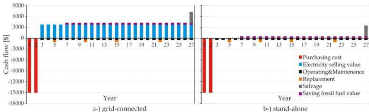
Fig. 8. Sample cash flows of PV systems
