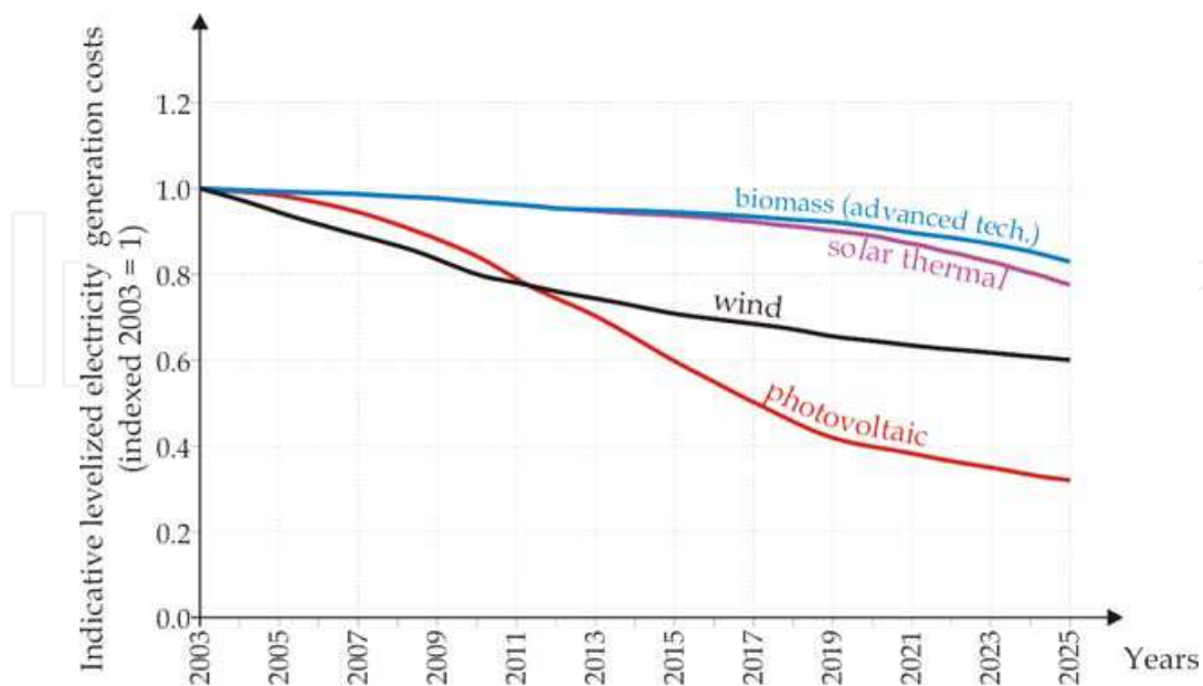
Fig. 3. Unit energy cost estimations of advanced energy generation technologies
