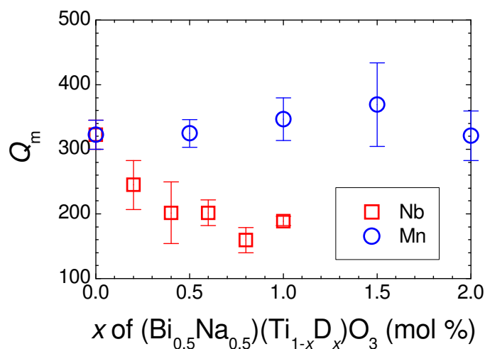
Fig. 5. Mechanical quality factor ( Q_m ) of (\text{Bi}_{0.5}\text{Na}_{0.5})(\text{Ti}_{1-x}\text{D}_x)\text{O}_3 ceramics (D = Nb, Mn)
