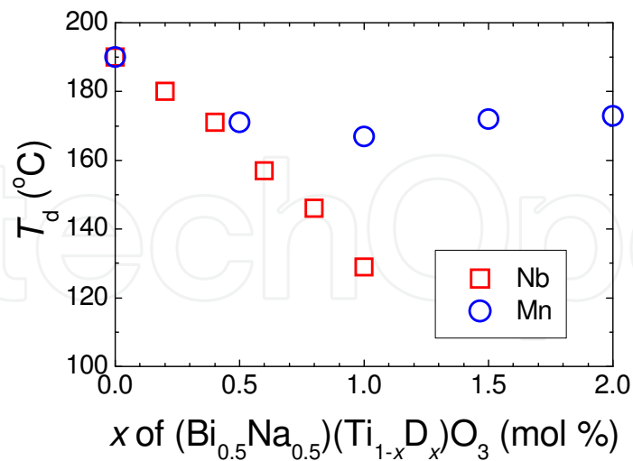
Fig. 7. Depolarization temperature ( T_d ) of (\text{Bi}_{0.5}\text{Na}_{0.5})(\text{Ti}_{1-x}\text{D}_x)\text{O}_3 ceramics ( D = \text{Nb, Mn} )
