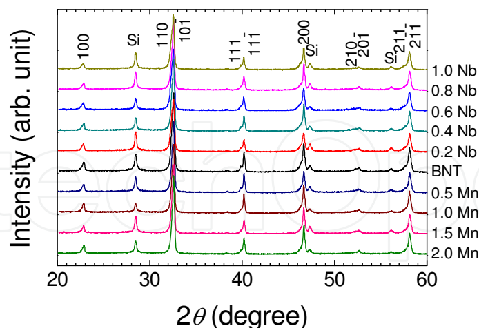
Fig. 1. XRD patterns of (\text{Bi}_{0.5}\text{Na}_{0.5})(\text{Ti}_{1-x}\text{D}_x)\text{O}_3 ceramics (D = Nb, Mn) sintered at 1150 °C for 2 h in air. Si peaks are of 5 N silicone powder used as an internal standard for calibration
