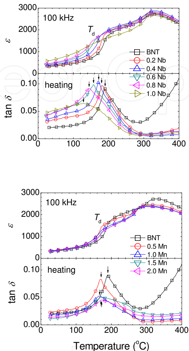
Fig. 6. Dielectric constant ( \epsilon ) and loss tangent ( \tan \delta ) of (\text{Bi}_{0.5}\text{Na}_{0.5})(\text{Ti}_{1-x}\text{D}_x)\text{O}_3 ceramics ( \text{D} = \text{Nb, Mn} ). Arrow marks indicate the depolarization temperature ( T_d )
