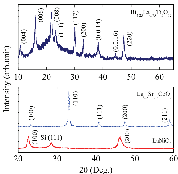
Fig. 1. The XRD patterns of \text{Bi}_{3.25}\text{La}_{0.75}\text{Ti}_3\text{O}_{12} , LNO and \text{La}_{0.5}\text{Sr}_{0.5}\text{CoO}_3 films, respectively.
