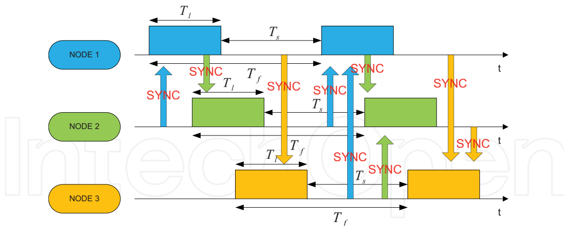
Fig. 4. STAR MAC Protocol Synchronization Messages Exchange
