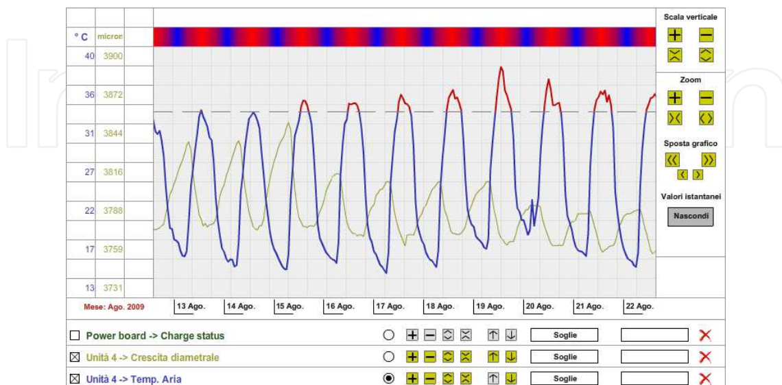
Fig. 9. Plant Diametric Trend vs. Air Temperature
