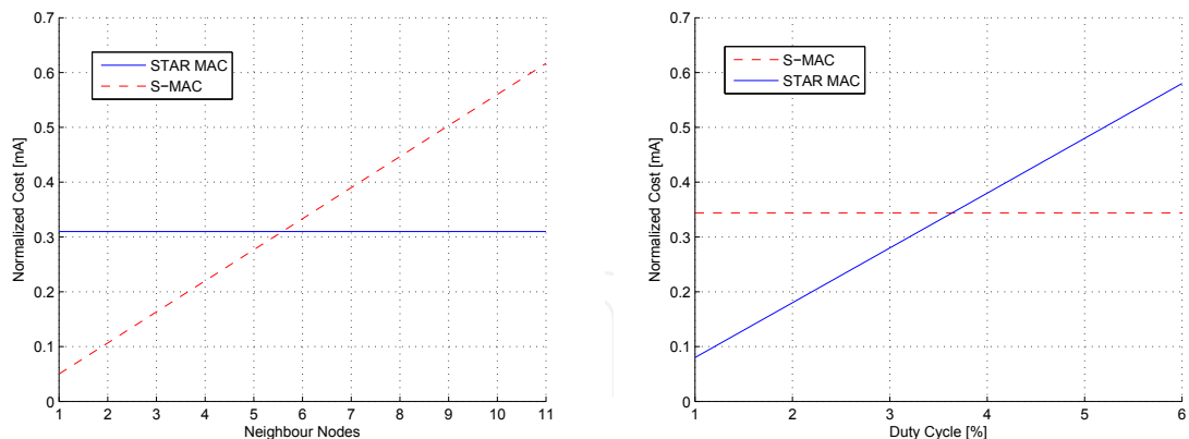
(a) Normalized Cost vs. Neighbor Nodes
