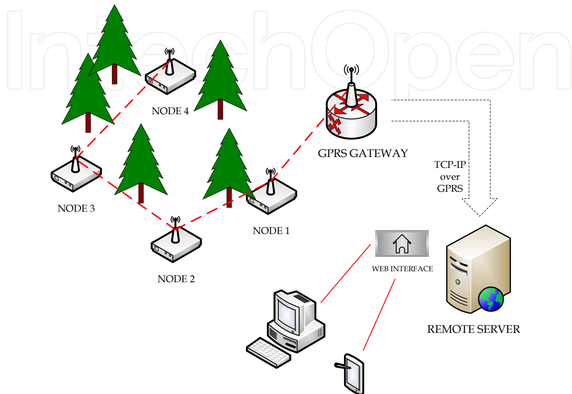
Fig. 1. Wireless Sensor Network System
