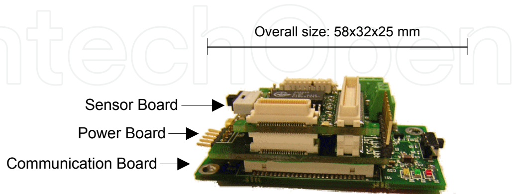
Fig. 2. Node Stack Architecture
