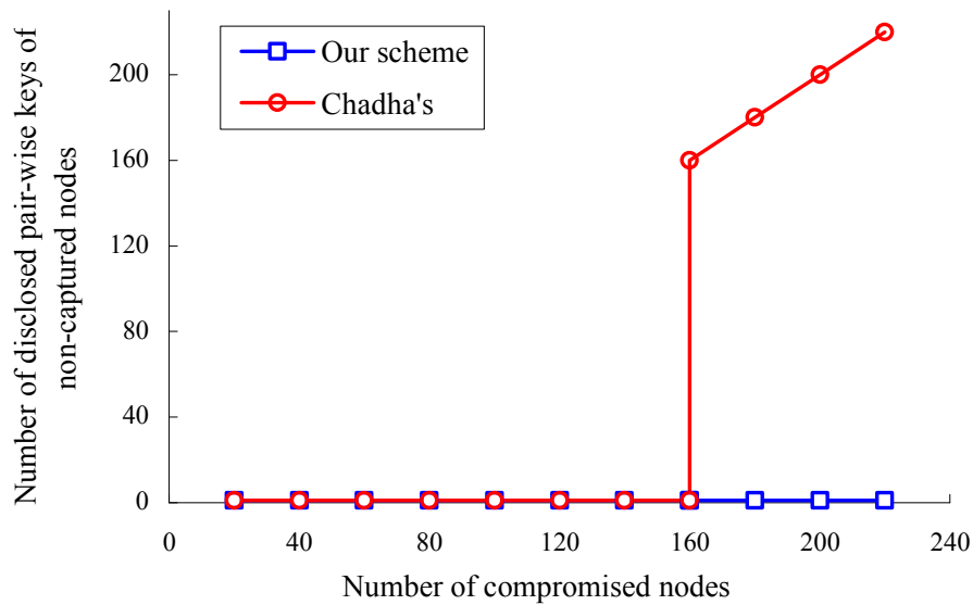
Fig. 5. NCA robustness comparison ( t = 80 )
