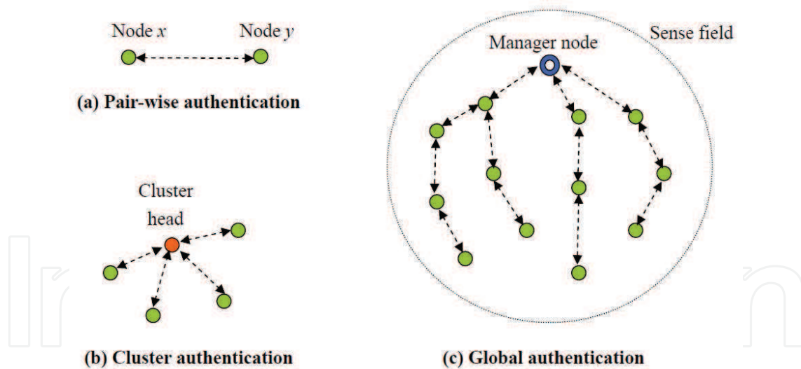
Fig. 2. Authentication scenarios
