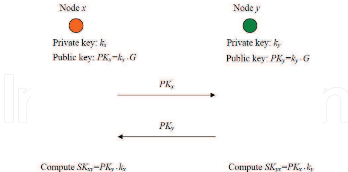
Fig. 3. Key exchange of a agreed pair-wise key under Diffie-Hellman based on ECDLP
