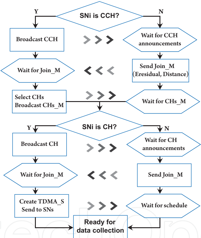
Fig. 6. Flowchart of CGC procedure
