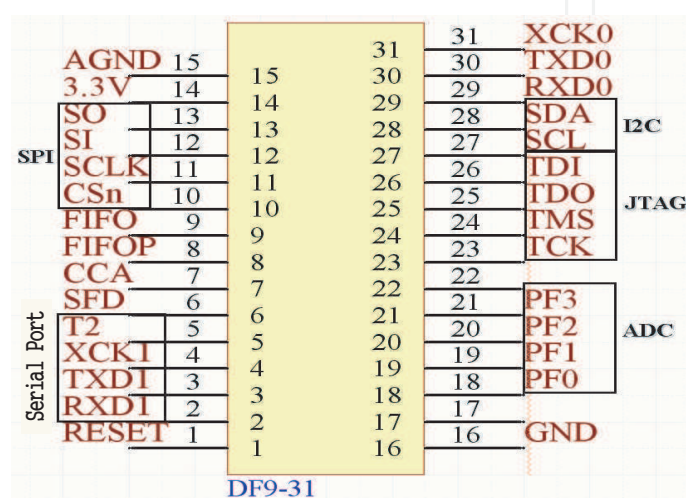
Fig. 12. Interface module schematic of the connector module
