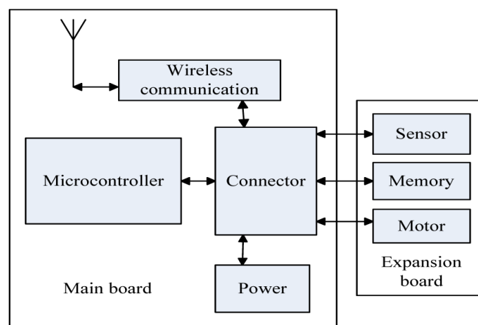
Fig. 11. Hardware architecture of the sensor node
