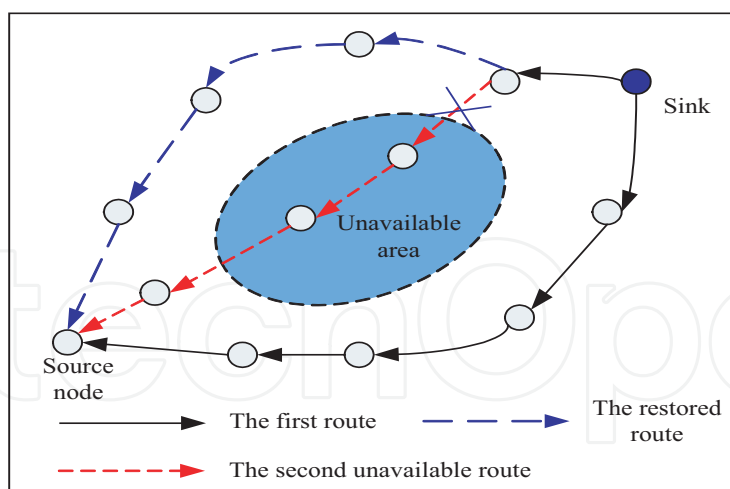
Fig. 10. Route Reply Procedure
