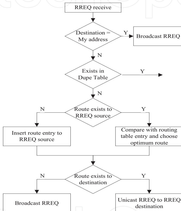
Fig. 7. Receive routing request
