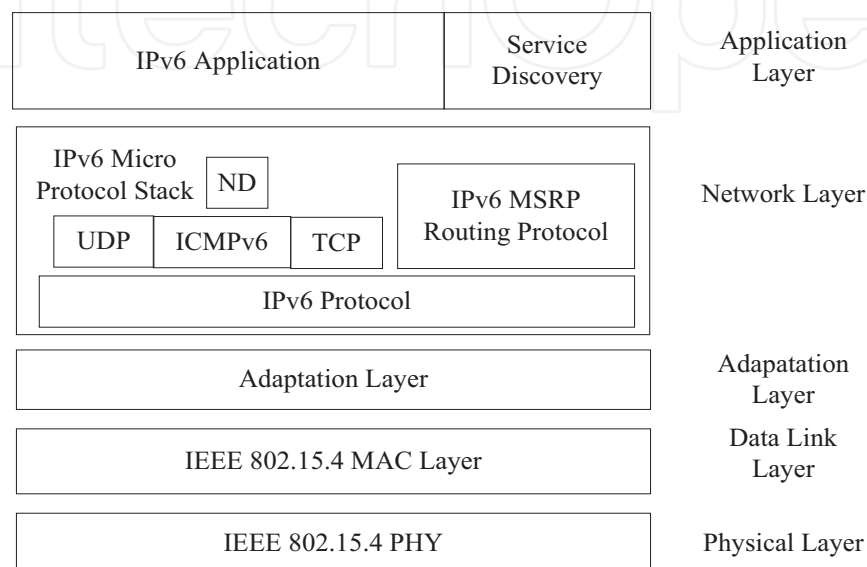
Fig. 1. Architecture of IPv6 Wireless Sensor Node
