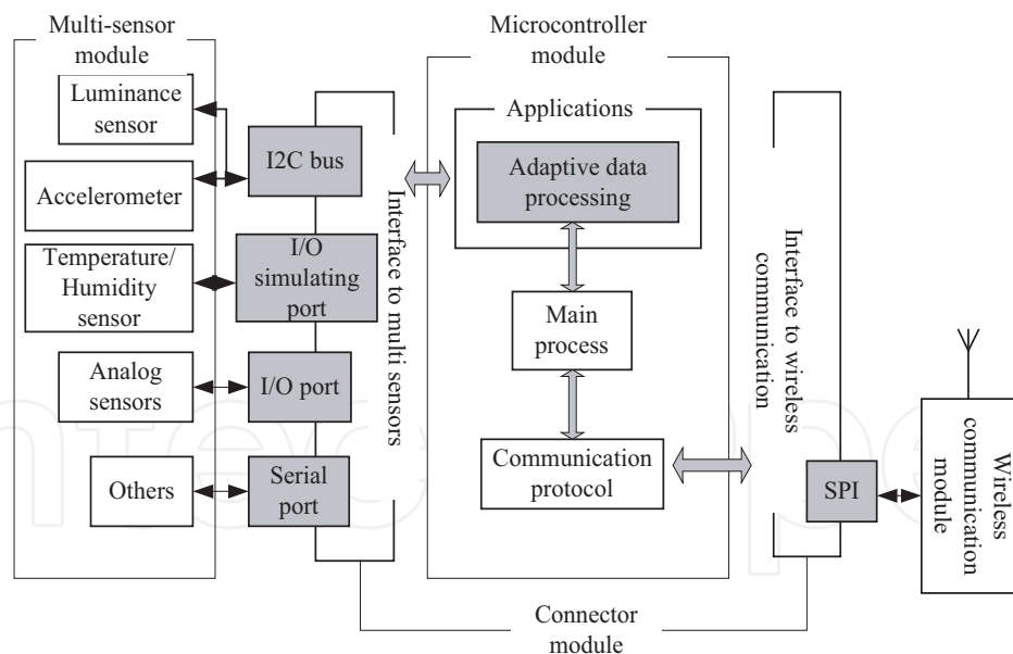
Fig. 16. Software framework of the sensor node
