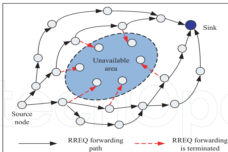
Fig. 9. RREQ message forwarding procedure
