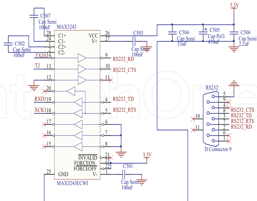
Fig. 13. Serial port schematic
