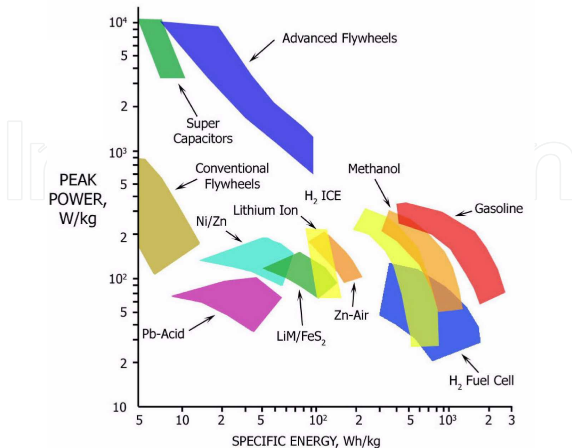
Fig. 6. Ragone plot for comparing the energy storage technologies and their power density versus energy density characteristics Tester (2005)
