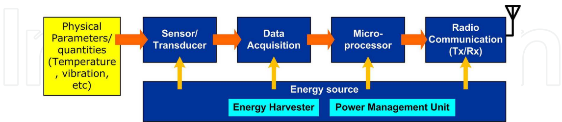
Fig. 4. Block diagram of energy-hungry wireless sensor node
