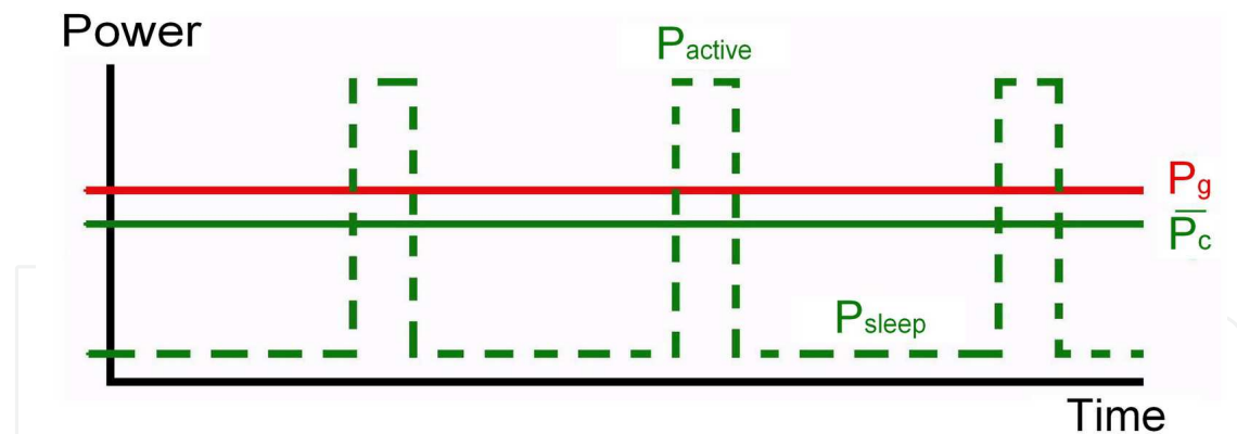
Fig. 11. Burst power consumption by the sensor node when P_{active} > P_g
