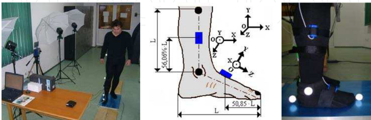
Fig. 14. Acquiring and measuring system, Biopac type, for the foot and lower leg linear accelerations
