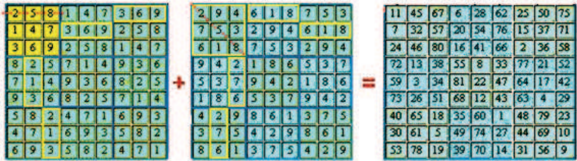
Fig. 3. Sudoku 9x9 from 3x3 square and bi-magic square (www.multimagie.com, 2009)
