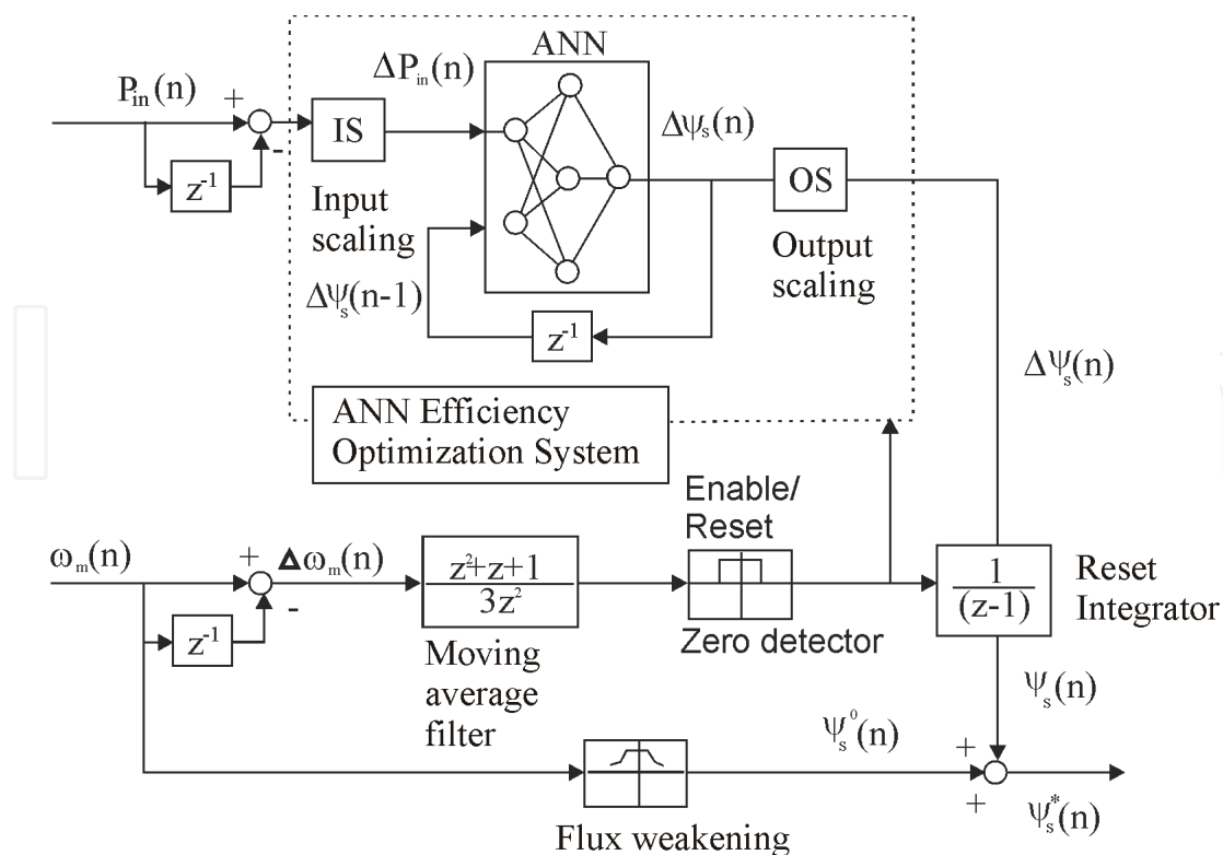
Fig. 10. ANN efficiency optimizer
