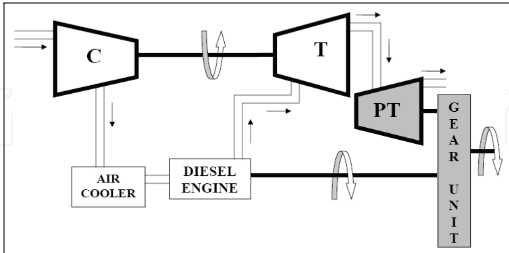
Fig. 1. Schematic view of Mechanical Turbocompounding.
