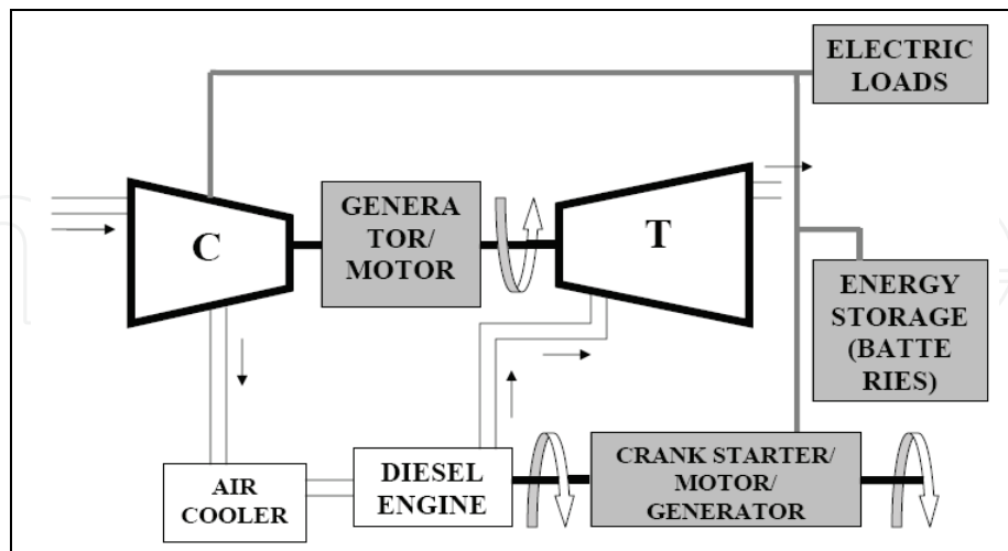
Fig. 7. Schematic view of Electrical Turbocharging.
