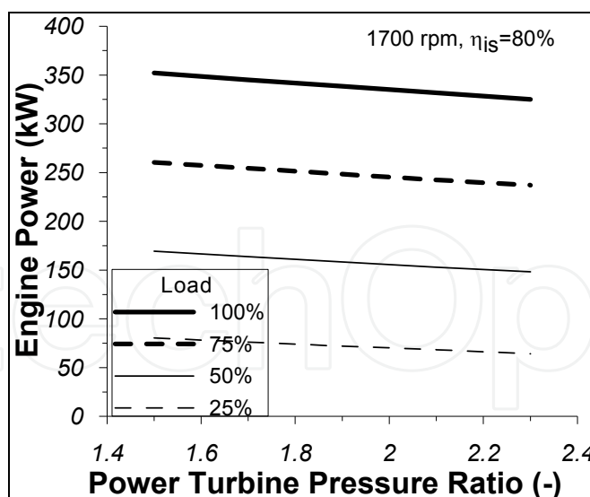
Fig. 5. Net engine power vs. power turbine pressure ratio at 1700 rpm and various engine loads.
