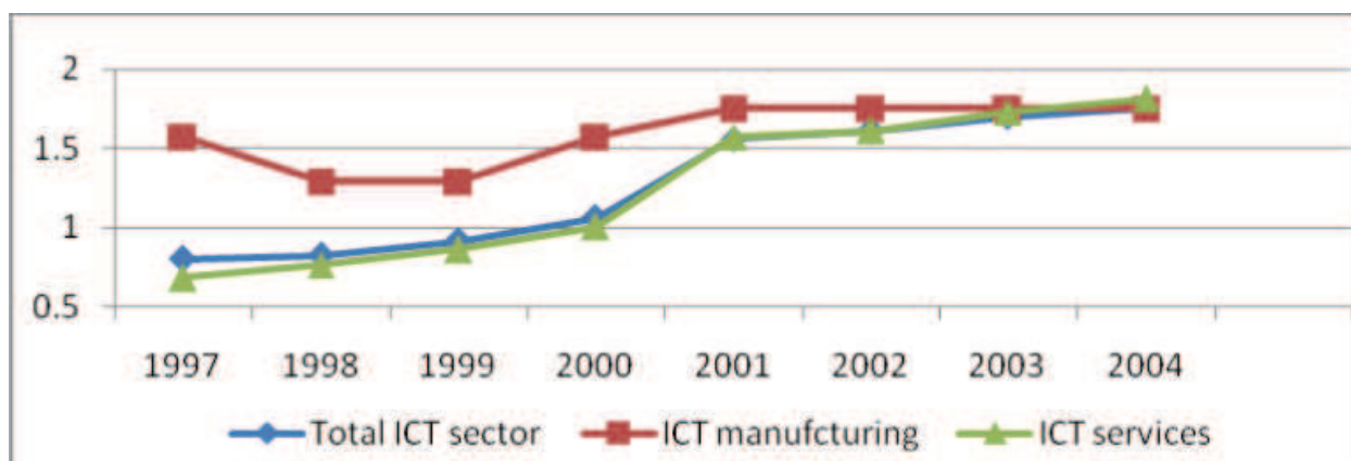
Fig. 1. Productivity coefficient trends in the total ICT sector, ICT manufacturing and ICT services (1997-2004)
