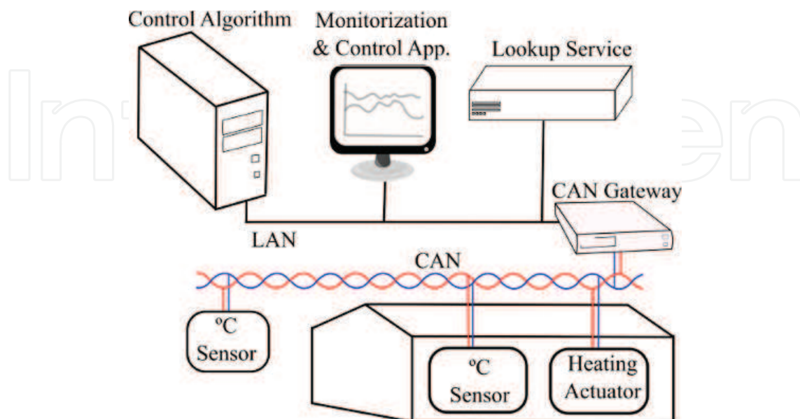
Fig. 12. Testing scenario used to control and monitor a greenhouse air temperature.
