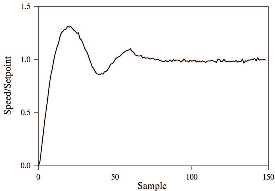
Fig. 15. P.I.D. Control of the DC shunt motor rotation speed.
