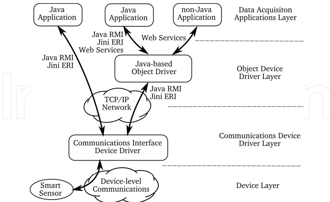
Fig. 1. Generic model for Java-based networked data acquisition systems.
