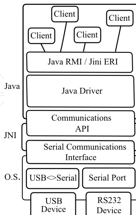
Fig. 2. Low-level Java-based device driver layered model
