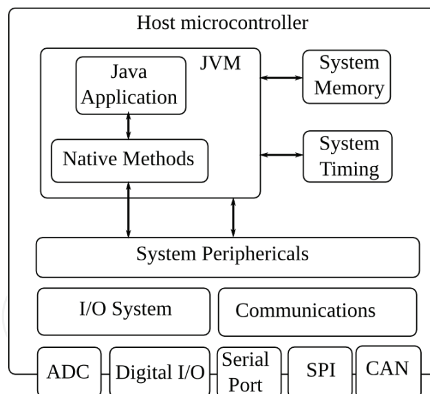
Fig. 8. Embedded Java Virtual Machine diagram block.
