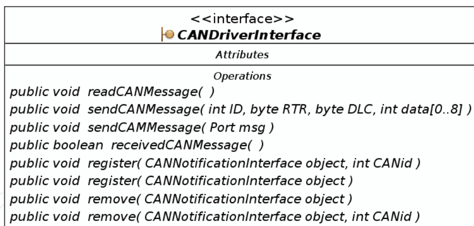
Fig. 3. CAN Driver Interface definition, which must be implemented by all drivers.
