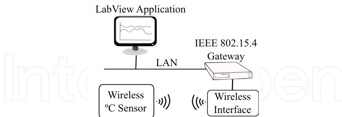
Fig. 10. Testing scenario used to monitor the air temperature using a wireless sensor.
