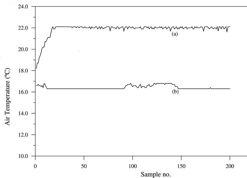
Fig. 13. P.I.D. temperature control of a miniature model of a greenhouse: a) temperature inside the greenhouse; b) temperature outside the greenhouse.
