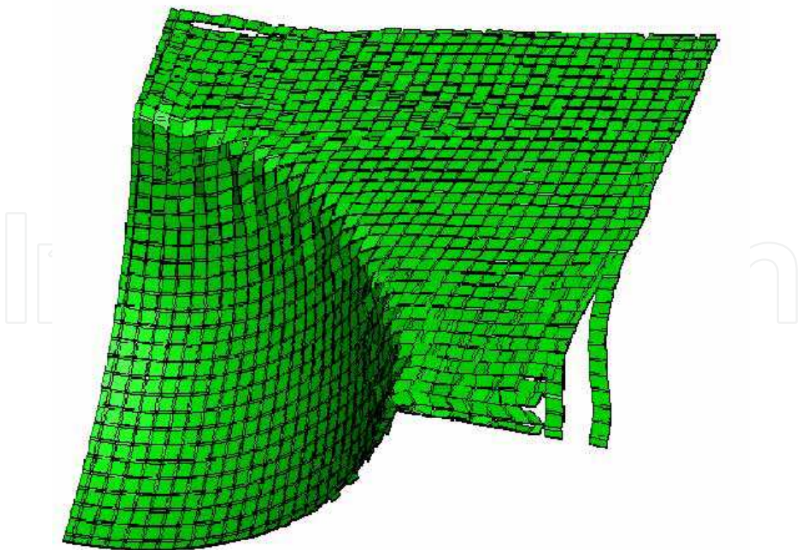
Fig. 18. Simulation of hemispherical forming test using the unit cell model of figure 16(b)
