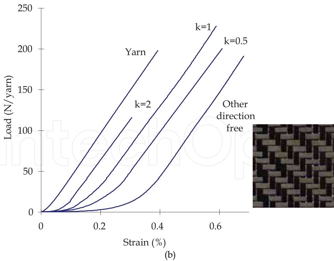
Fig. 6. (a) Biaxial tensile test on cross-shaped specimen (b) Load versus strain for carbon twill weave. k = \epsilon_{warp} / \epsilon_{weft} (Buet-Gautier et al, 2001)
