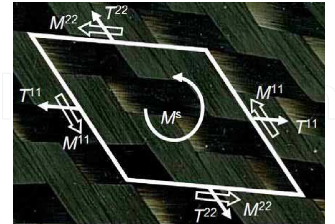
Fig. 19. Unit woven cell submitted to tension, in plane shear and bending
