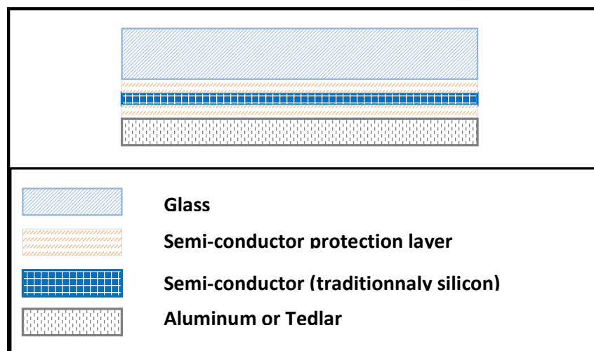
Fig. 3. Cross section of a typical photovoltaic panel
