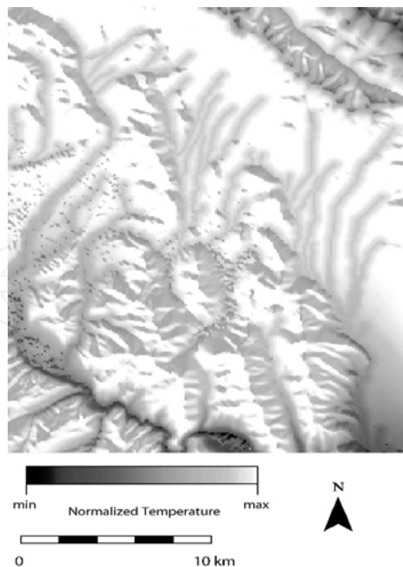
Fig. 6. Normalized temperature with values from 0 to 255.
