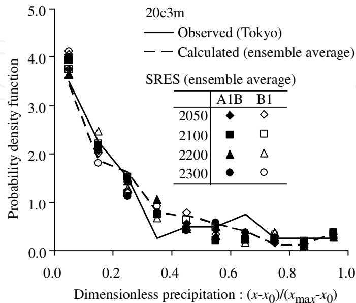
Fig. 6. Frequency distribution of precipitation in the PDS.
