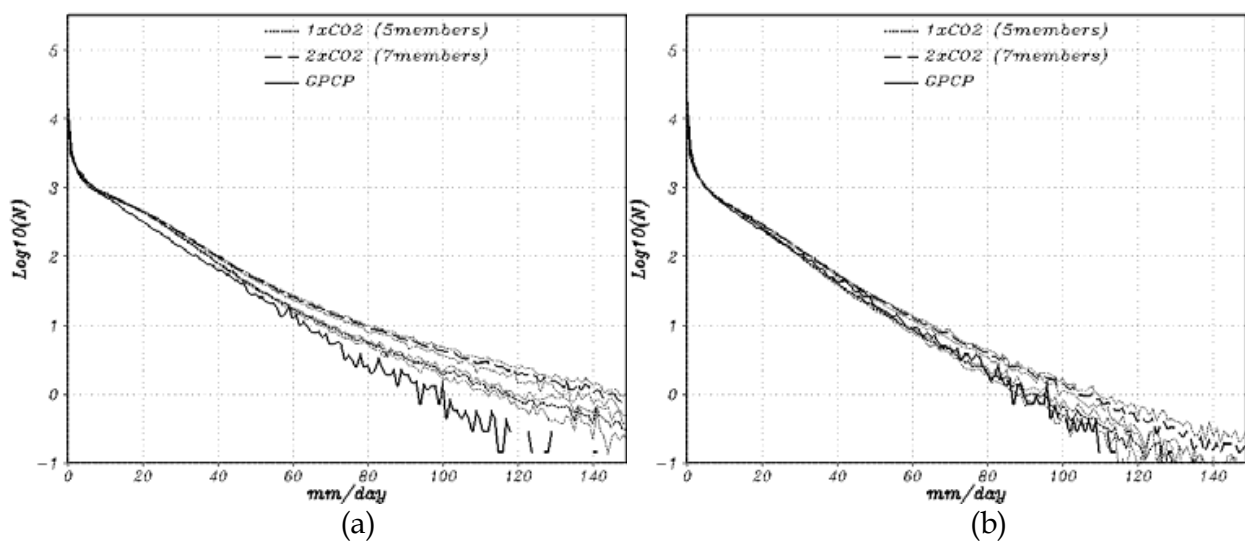
Fig. 2. Frequency distribution of daily precipitation over land of (a) South Asia (8.5°–30°N, 65°–100°E) and (b) China (20°–40°N, 100°–130°E) during JJAS. Solid lines show observations from the GPCP 1DD (1997–2003). The short dashed line and long dashed line denote the ensemble average from the control and 2 × CO 2 experiments. Thin dashed lines show the standard deviation of each ensemble.
