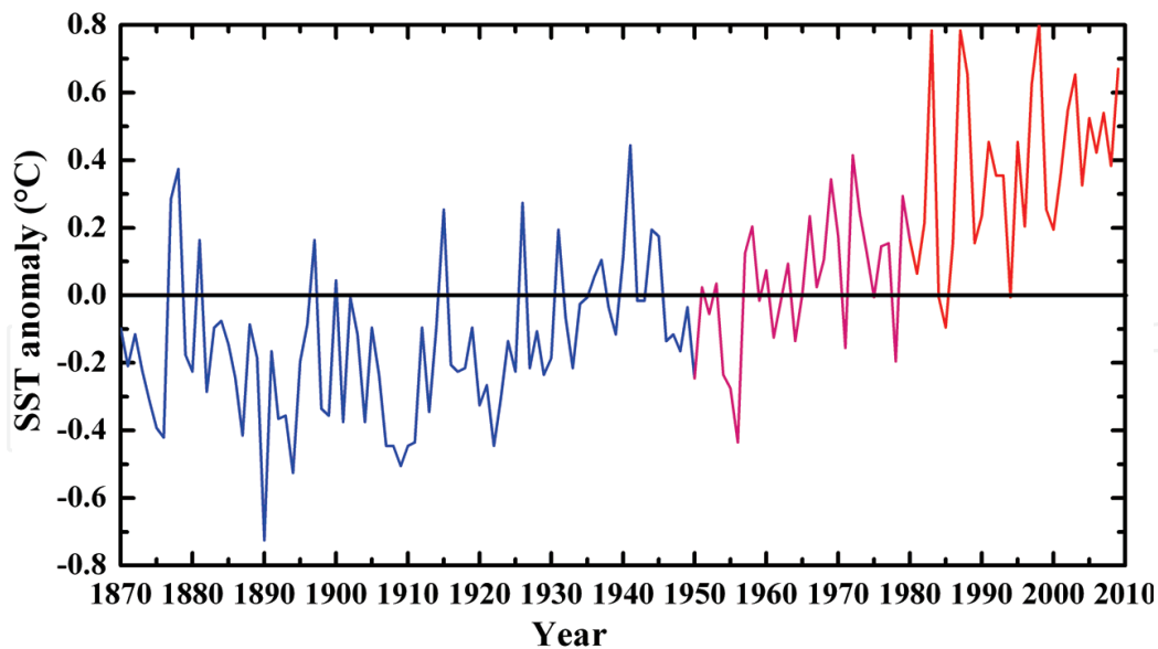
Fig. 1. SST anomaly over the NIO (40°E - 100°E, 5°N - 25°N) during southwest monsoon season. Blue, pink and red colour indicates 1870 - 1949, 1950 - 1980 and 1981 - 2009 respectively.
