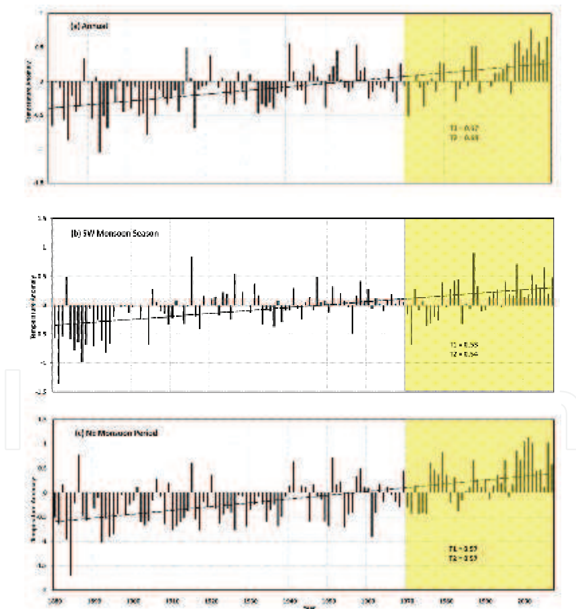
Fig. 5. Variation of all India surface-air-temperature (Dashed line is trend; T1-trend for 1880-2006, T2-trend for 1970-2006).
