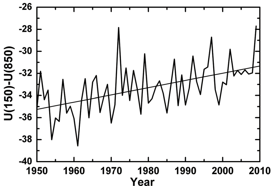
Fig. 2. Vertical wind shear (m/s) of zonal wind during southwest monsoon season over the North Indian Ocean.
