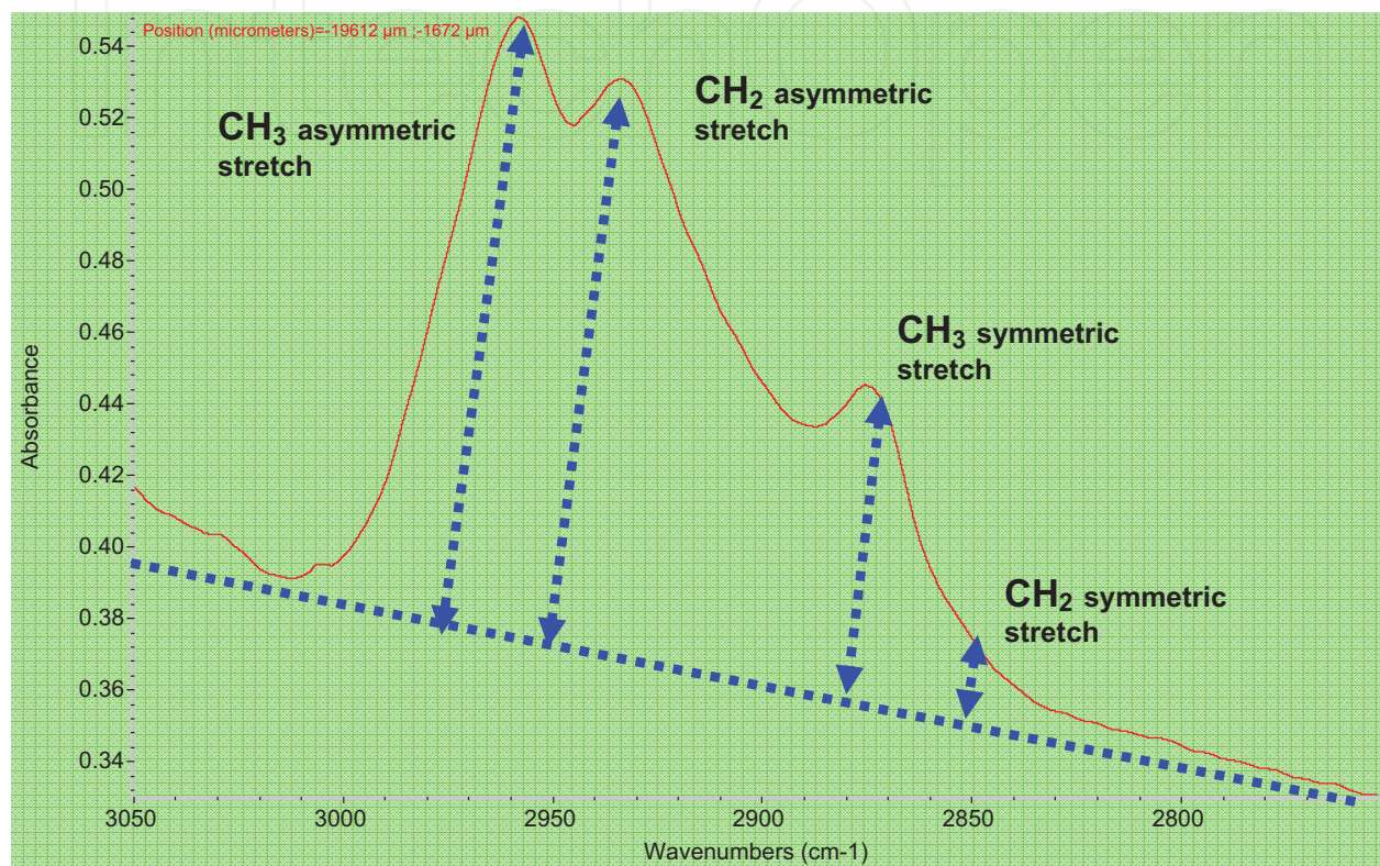
Fig. 2. The \text{CH}_2 and \text{CH}_3 asymmetric and symmetric stretching band features in typical ultra-spatially resolved synchrotron-based FTIRM spectrum in plant tissue (aleurone tissue of sorghum, pixel size: 10 \mu\text{m} \times 10 \mu\text{m} ) in the C-H stretch region ca. 3015\text{--}2780 \text{ cm}^{-1} showing C-H function groups of biopolymers in complex plant tissue system: \text{CH}_3 asymmetric stretch at ca. 2958 \text{ cm}^{-1} , \text{CH}_2 asymmetric stretch at ca. 2934 \text{ cm}^{-1} , \text{CH}_3 symmetric stretch at ca. 2874 \text{ cm}^{-1} , and \text{CH}_2 symmetric stretch at ca. 2851 \text{ cm}^{-1} .
