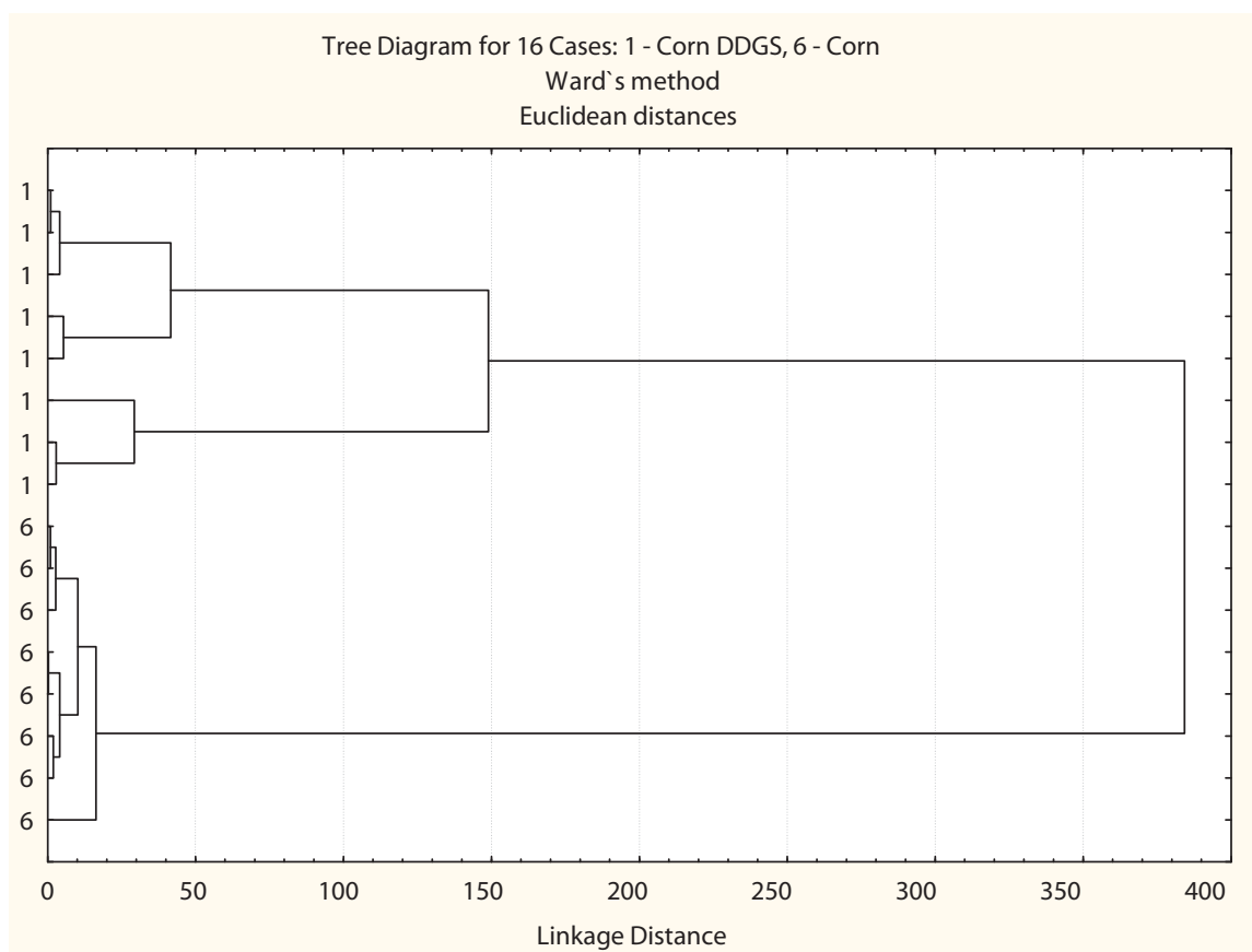
Fig. 5. Cluster analysis of spectrum detected with DRIFTS (acquired at 4 cm -1 resolution in the reflectance mode with subtraction of the KBr background, accumulated 256 times; range of wavenumbers, 3027-2813 cm -1 , IR reflectance Kubelka-Munk units) obtained from corn DDGS (1) vs. corn grain (6) from all original spot spectrum [CLA: (a) region of CH groups (CH 2 , CH 3 ) ca. 3027-2813 cm -1 ; (b) distance method, Euclidean; (c) cluster method, Ward's algorithm] (source: D. Damiran)
