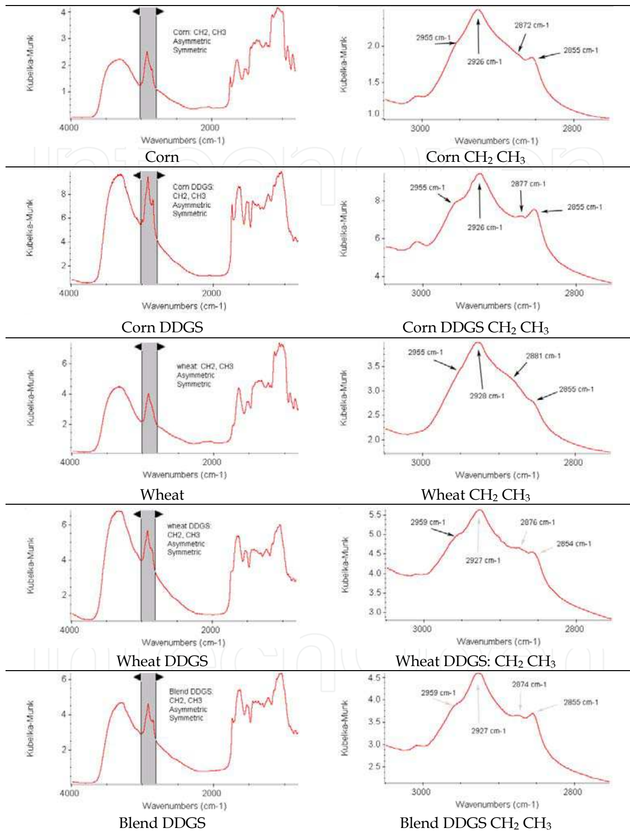
Fig. 4. Comparison of different types of DDGS and original feedstock in \text{CH}_3 and \text{CH}_2 asymmetric and symmetric stretching bands profiles using the DRIFT molecular spectroscopy: Effect of Bio-Ethanol Processing
