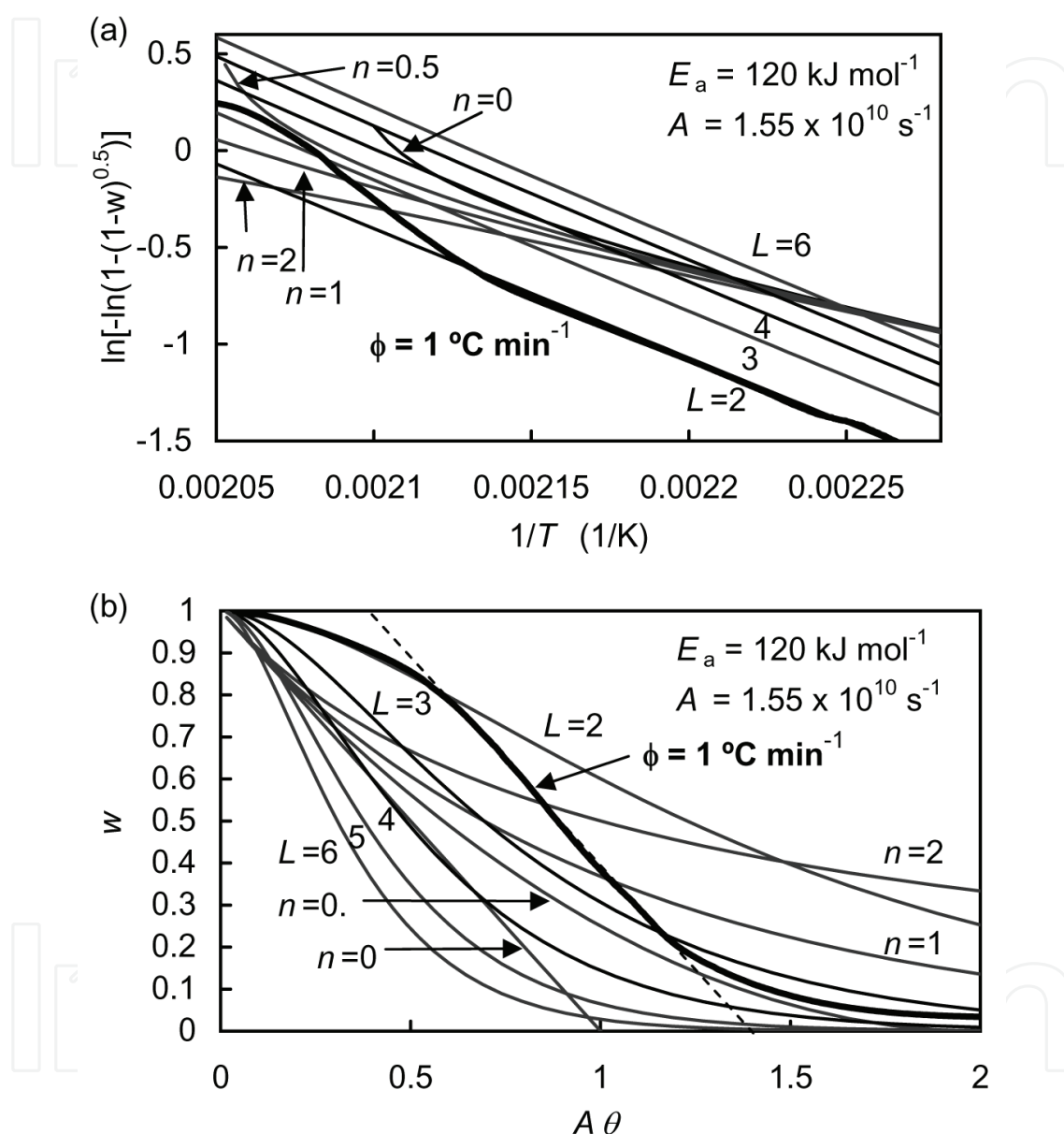
Fig. 4. Plots of (a) \ln[-\ln\{1-(1-w)^{0.5}\}] vs. 1/T and (b) w vs. A\theta for thermogravimetric data of PHB/MgO (100:5 wt/wt) at a heating rate of 1 \text{ °C min}^{-1} ( E_a=120 \text{ kJ mol}^{-1} , A=1.55 \times 10^{10} \text{ s}^{-1} ), and for model reactions. Model reactions: zero ( n=0 ), half ( n=0.5 ), 1 st ( n=1 ), 2 nd -order ( n=2 ), and random degradations (random L=2-6 ).
