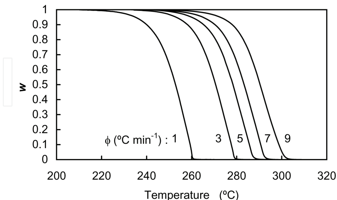
Fig. 1. TG curves of PHB degradation at multiple heating rates ( \phi=1, 3, 5, 7 and 9 °C min -1 ) in a constant N 2 flow (100 mL min -1 ).
