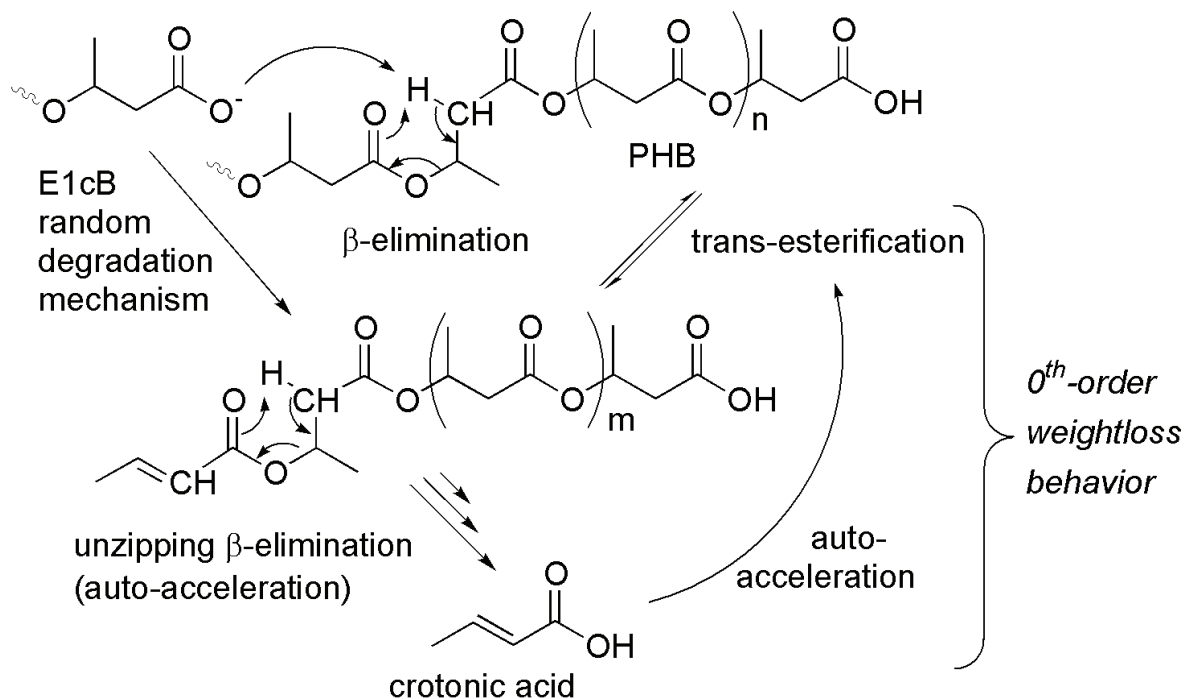
Scheme 2. Expected overall thermal degradation pathway of PHB.
