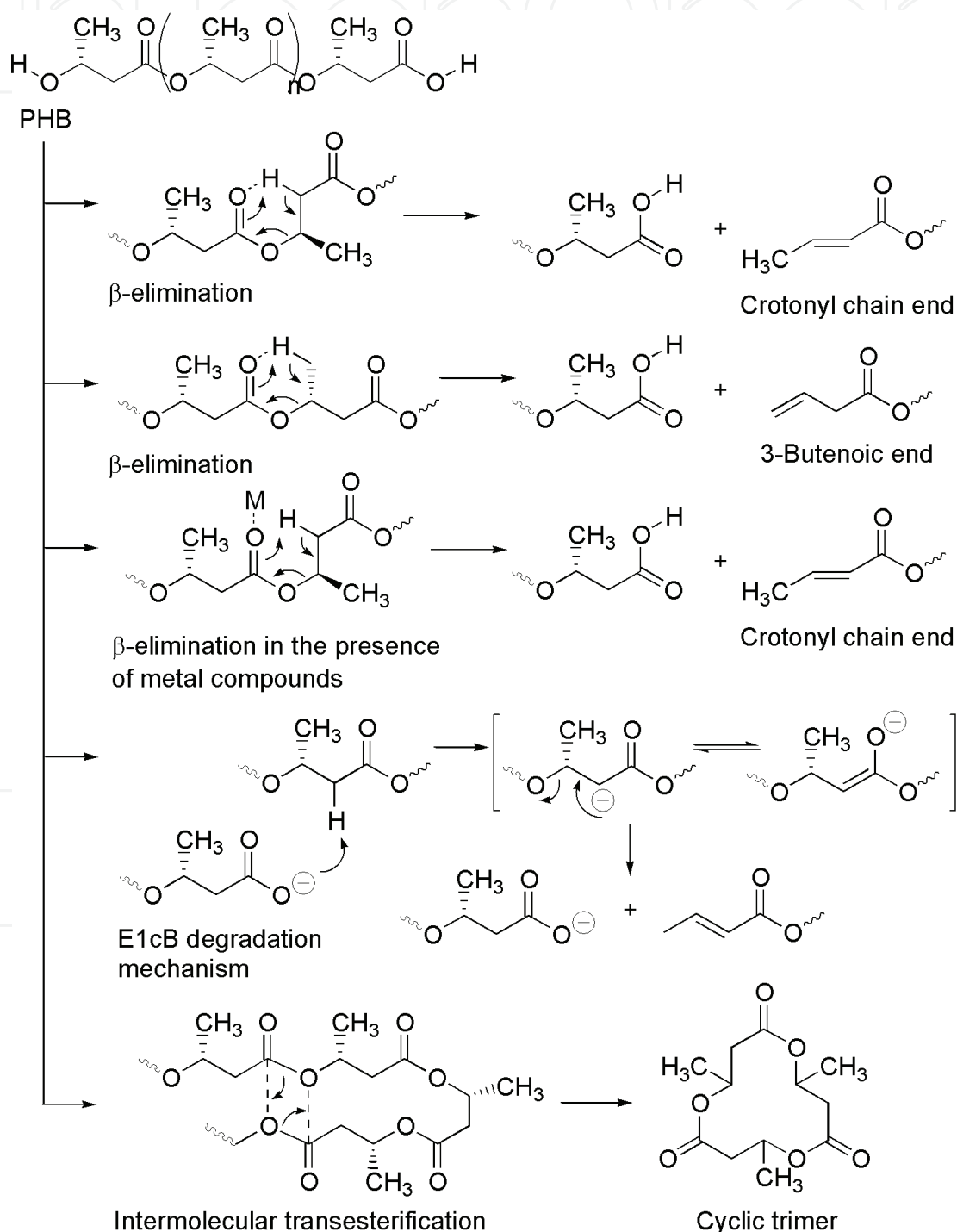
Scheme 1. Reported thermal degradation mechanisms of PHAs.
