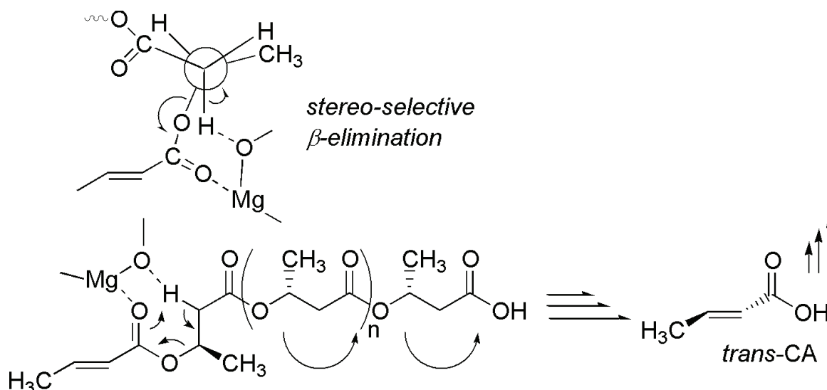
Scheme 3. Trans -form preferential depolymerization of PHB.
