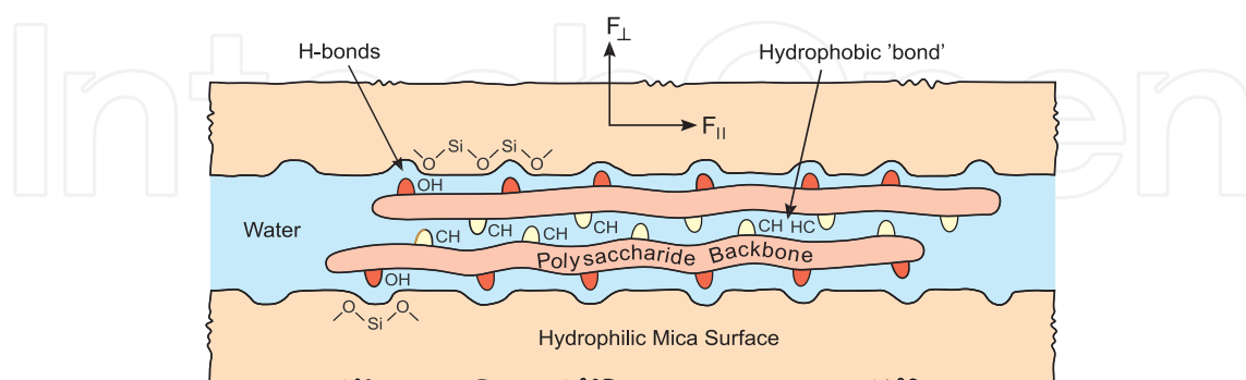
Fig. 7. Likely molecular mechanisms, involving confinement and shear-induced alignment of the polysaccharide molecules, allowing them to act as good lubricants and adhesives. Adapted from (Gourdon et al., 2008).
