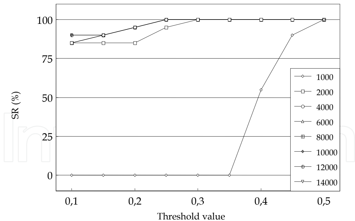
Fig. 11. Neural Networks Success Rate vs. threshold value for different numbers of learning steps.
