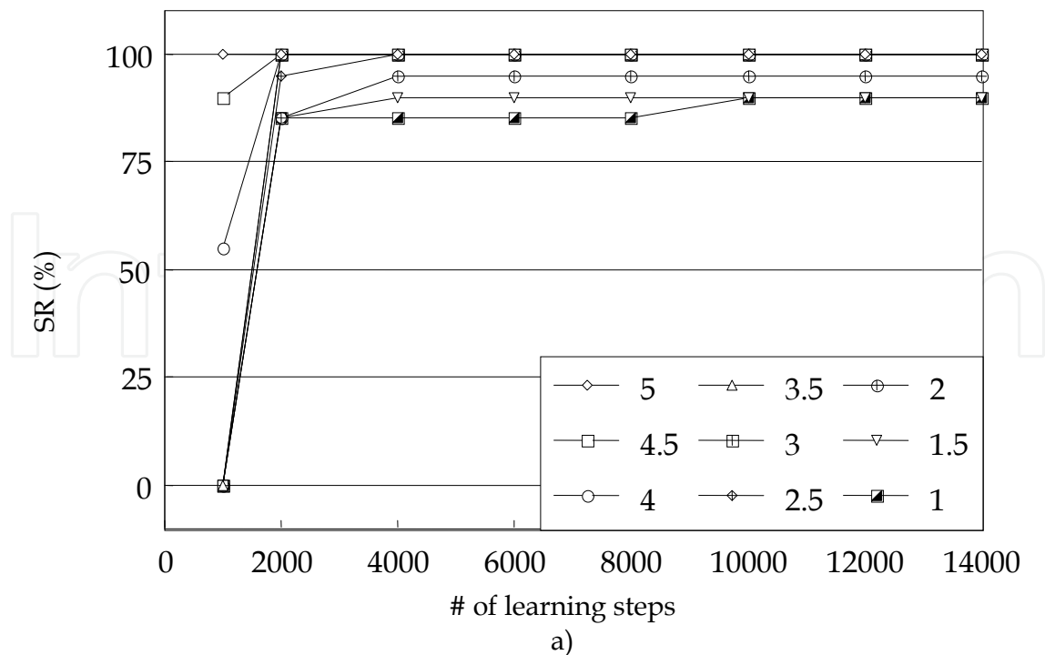
Fig. 10. Neural Network Success Rate vs. number of learning steps for different threshold values.
