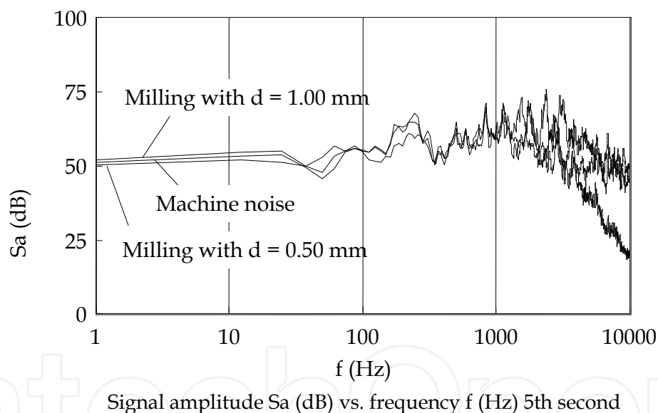
Fig. 2. Signal amplitude S_a (dB) vs. frequency f (Hz) of the audible sound signals for the 5th second of each test. Namely, milling with S = 800 rpm, f = 80 mm/min, d = 0.5 mm; milling with S = 800 rpm, f = 80 mm/min, d = 1 mm, and machine tool running unloaded at S = 800 rpm.
