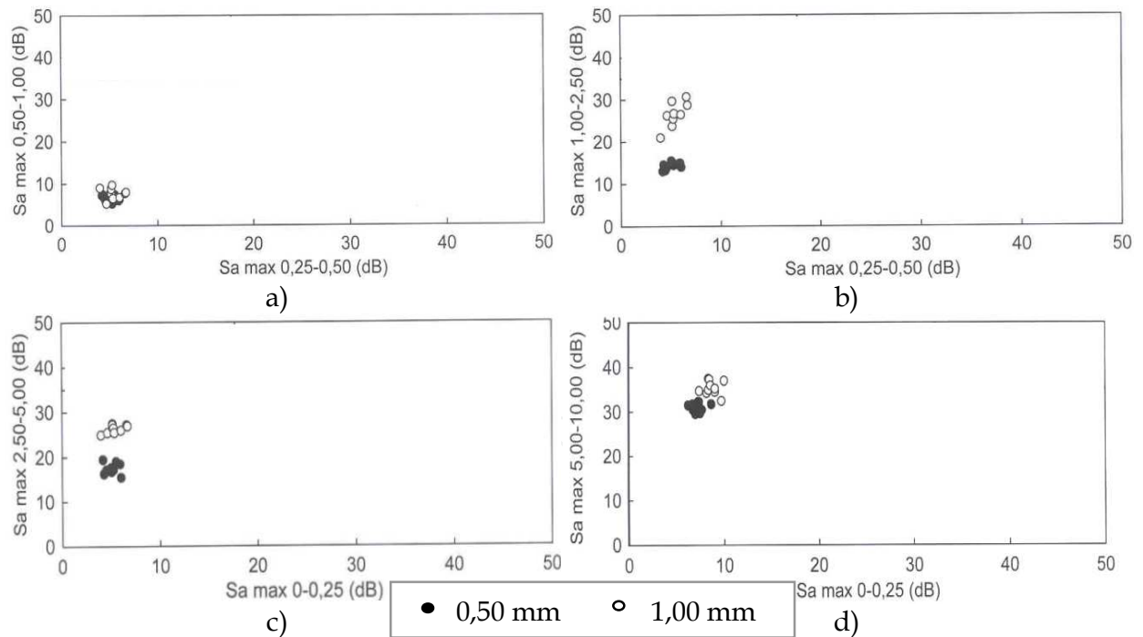
Fig. 6. Pair-wise plots of “difference signal” maximum amplitudes for medium frequency intervals.
