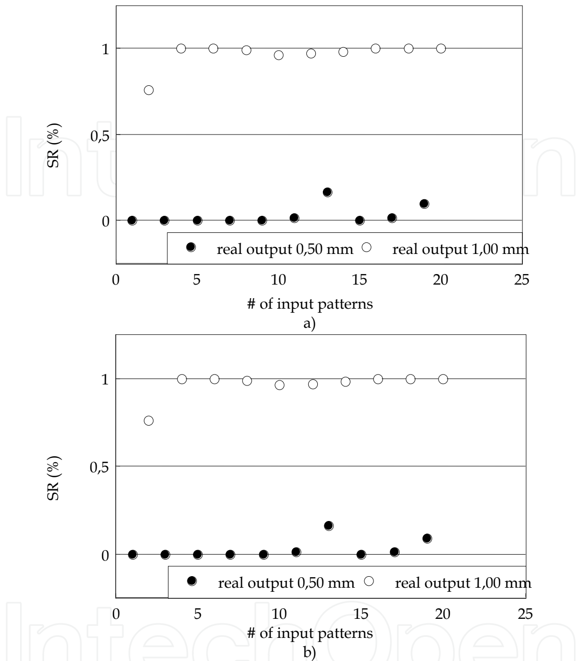
Fig. 9. Neural Network output vs. number of input patterns for: a) 12000 and b) 14000 learning steps.
