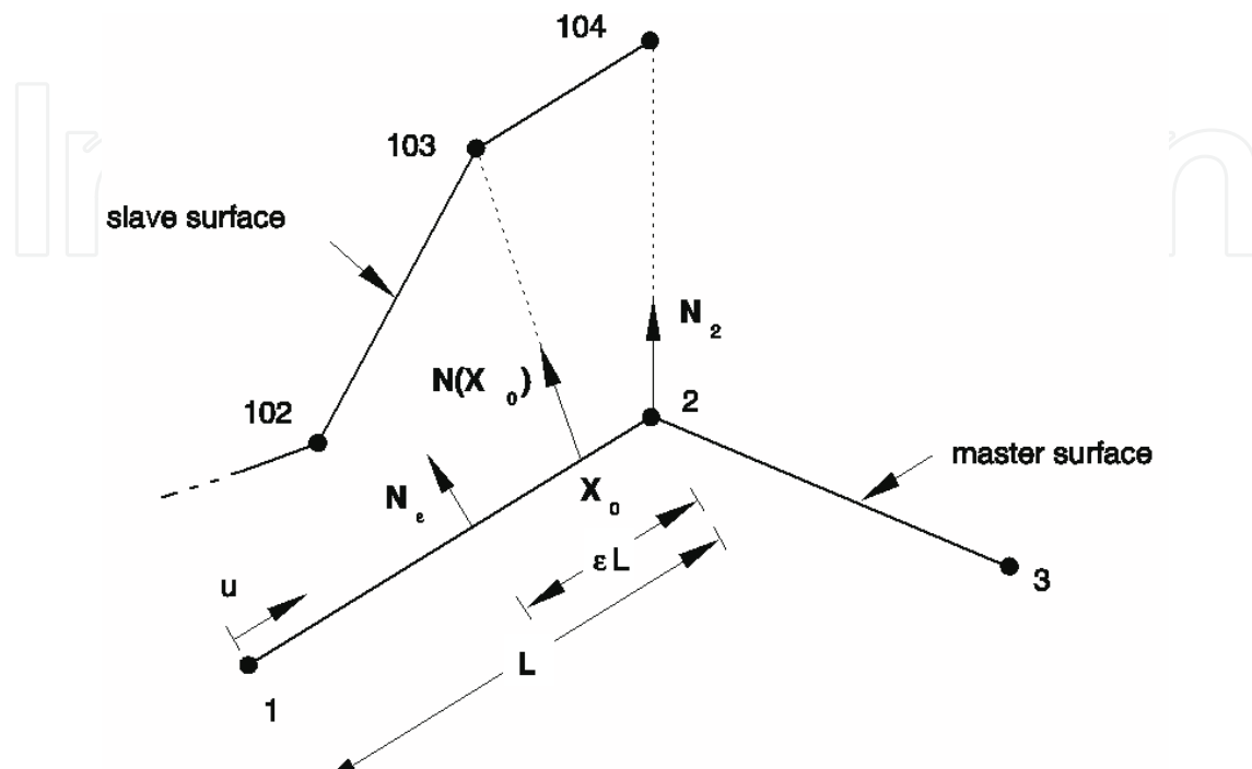
Fig. 2. Slave and master surfaces
