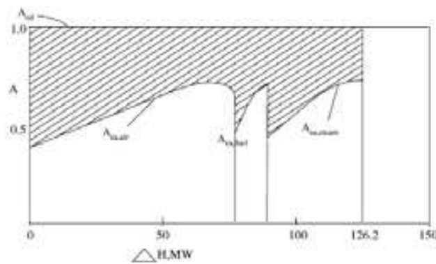
Fig. 6.5. Energy-utilization for the combustion chamber.
