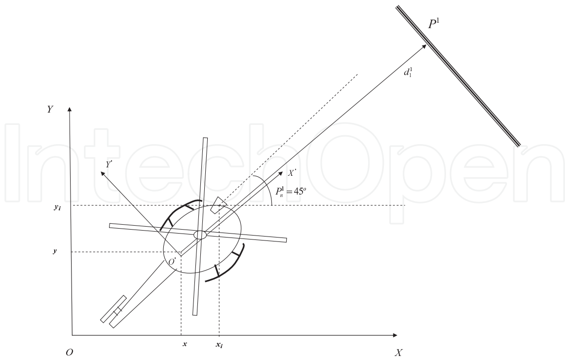
Fig. 10. Reference frames for the UAV
