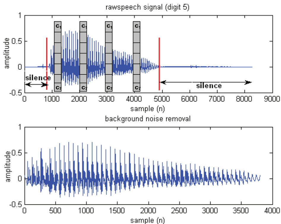
Fig. 7. This figure shows a raw speech signal sampled at 12 KHz for 8260 samples. The utterance can be divided in three clearly differentiable parts: silence, speech and then silence. The waveform has quite a significant part of silence in the beginning and the end of a signal. End-point detection technique removes the silence part from raw speech signal and only voiced portion of the signal as shown in the bottom plot is processed. By using an end point detection technique, overall processing time can be improved to 53%.
