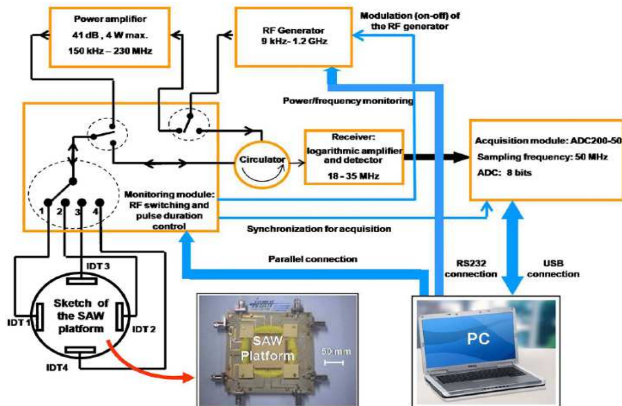
Fig. 17. Schematic diagram of SAW actuator system used for tracking microdroplet.
