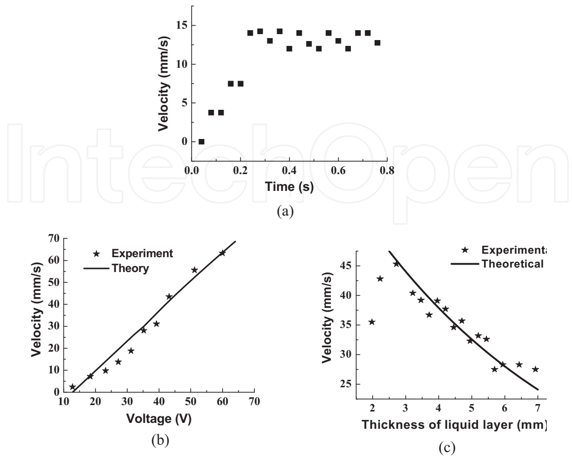
Fig. 13. Velocity of non-contact SAW linear motor: (a) transient velocity; (b) average velocity VS voltage; (c) average velocity VS thickness of liquid layer ( f=9.959 MHz)
