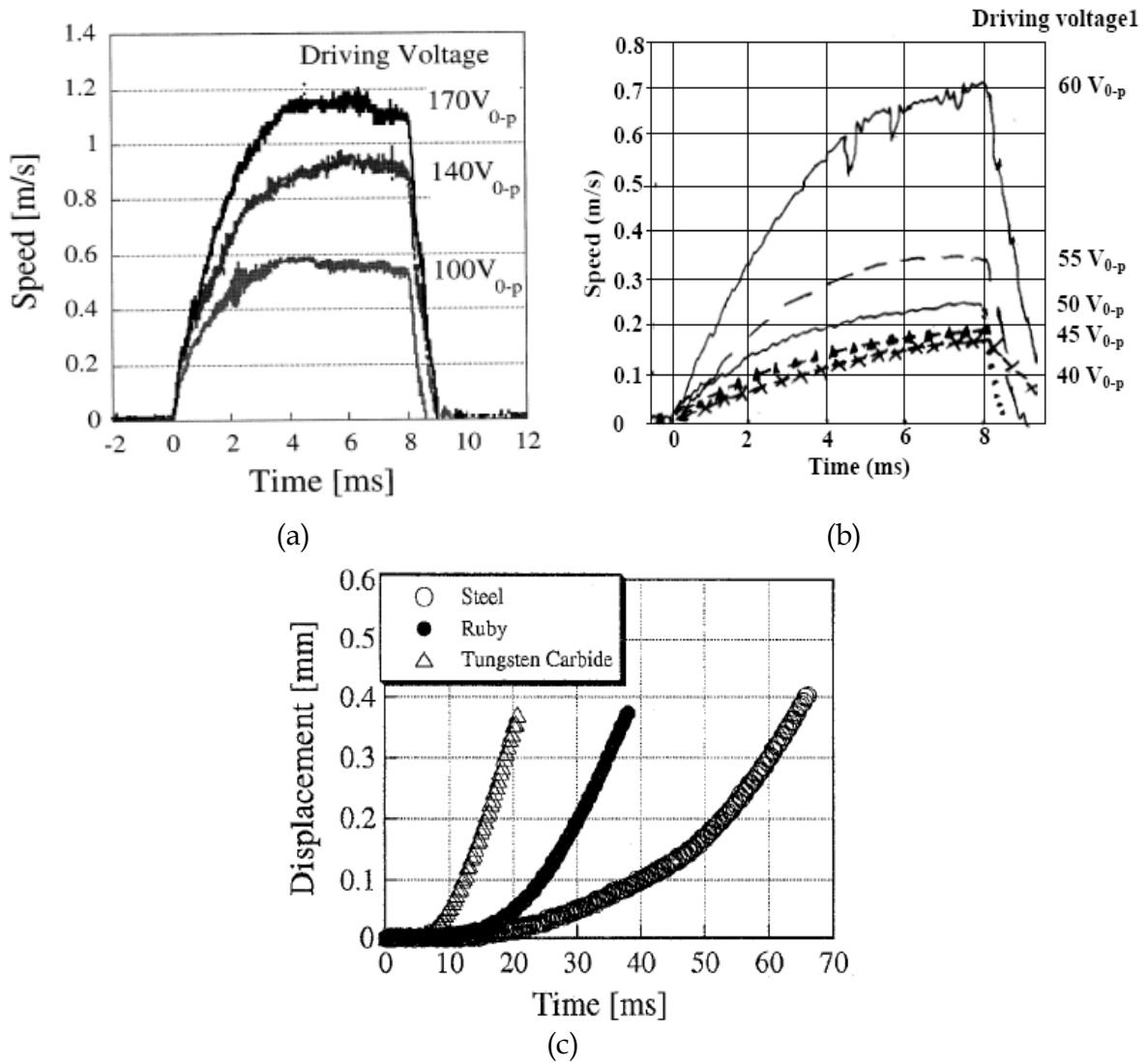
Fig. 4. Transient response of SAW motor: (a) at about 10 MHz; (b) at 50 MHz; (c) at about 10 MHz.
