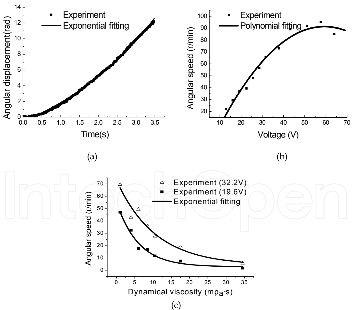
Fig. 14. Response of non-contact rotary motor: (a) angular displacement VS time; (b) angular speed VS voltage; (c) angular speed versus the dynamical viscosity of liquid layer
