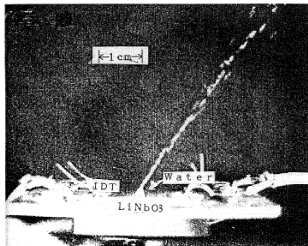
Fig. 10. Water jet streaming excited by SAW.
