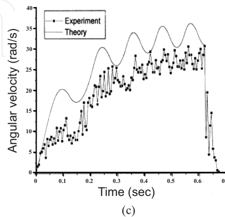
Fig. 9. Numerical simulations of rotary motors: (a) theoretical model; (b) angular displacement versus time; (c) angular velocity versus time.
