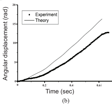
Fig. 9. Numerical simulations of rotary motors: (a) theoretical model; (b) angular displacement versus time; (c) angular velocity versus time.
