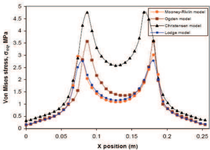
Fig. 10. Von Mises stress distribution, symmetry plan XZ
