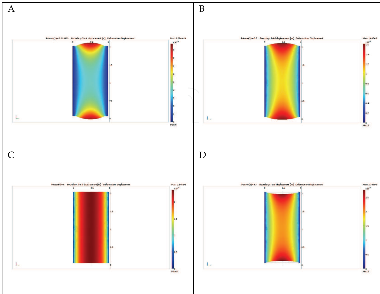
Fig. 5. YZ-view of total displacement of the box-1 for different Poisson's ratios: A) \nu = -0.999999 , B) \nu = -0.7 , C) \nu = 0 , D) \nu = 0.3
