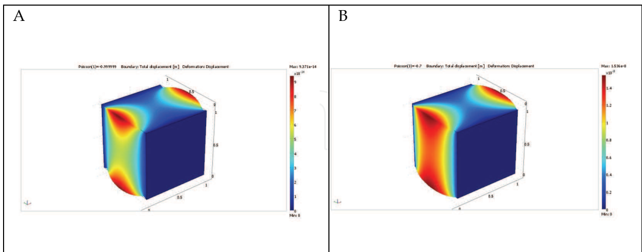
Fig. 5. YZ-view of total displacement of the box-1 for different Poisson's ratios: A) \nu = -0.999999 , B) \nu = -0.7 , C) \nu = 0 , D) \nu = 0.3
