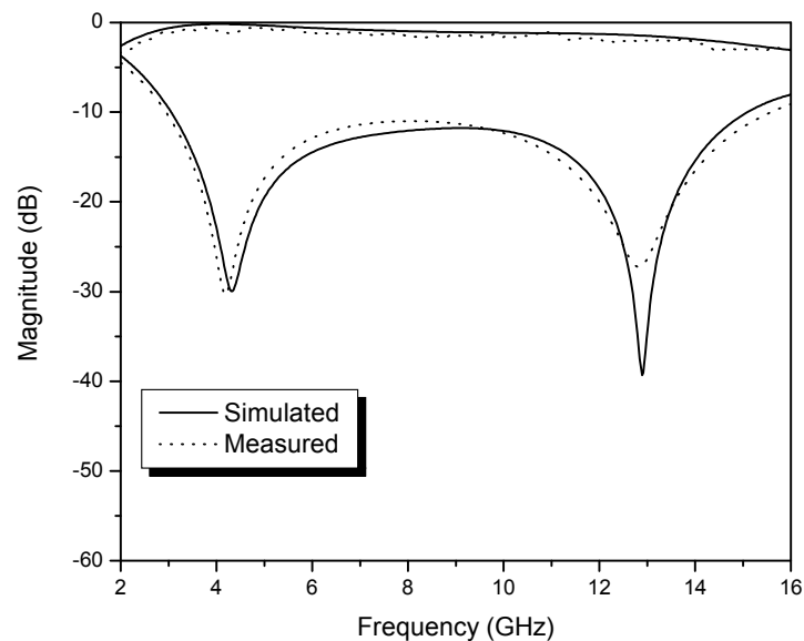
Fig. 2. Simulated and measured results of the UWB transition.
