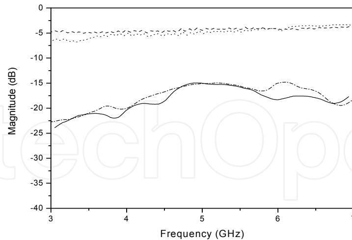
Fig. 19. Scattering parameters of the proposed coupler.
