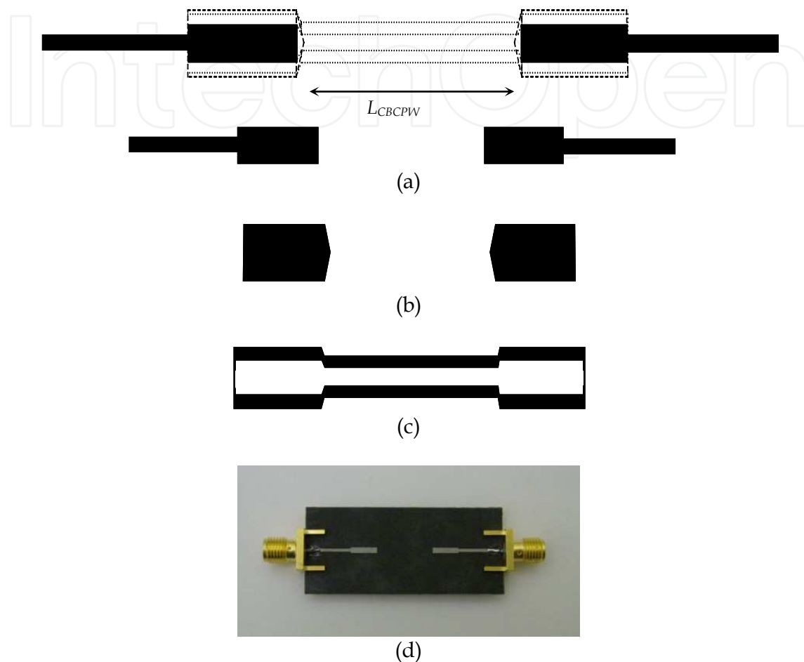
Fig. 9. Layout of the UWB filter (a) Top layer (b) Common slot in ground plane (c) Bottom layer (d) Fabricated filter.
