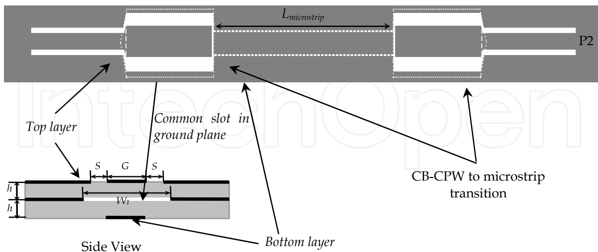
Fig. 5. Layout of the CBCPW fed UWB filter
