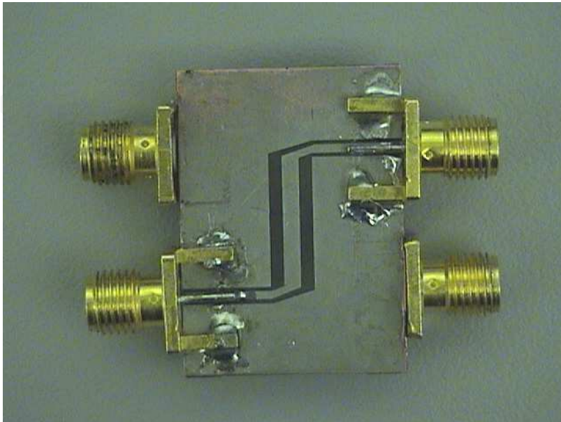
Fig. 18. Photograph of the fabricated circuit prototype
