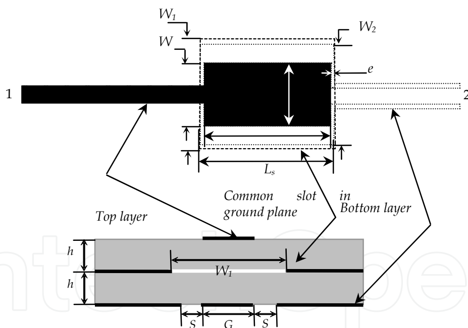
Fig. 1. Layout of the microstrip-to-CB-CPW transition.
