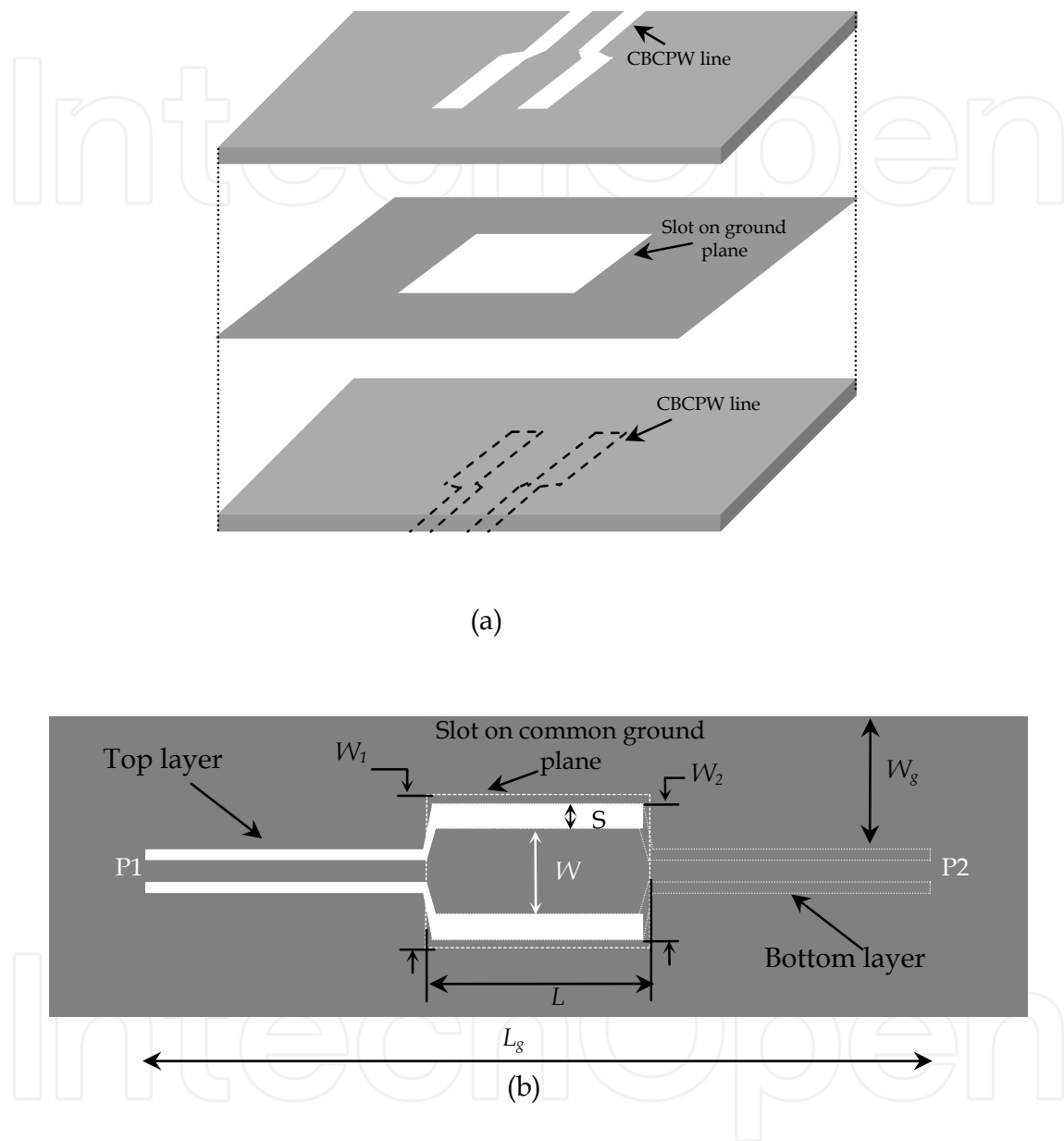
Fig. 3. Layout of the CB-CPW-to-CB-CPW transition.
