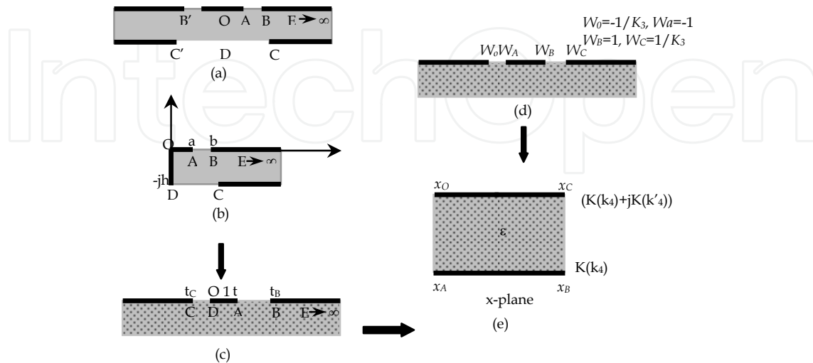
Fig. 14. Conformal mapping transformation of the even-mode in the dielectric region.
