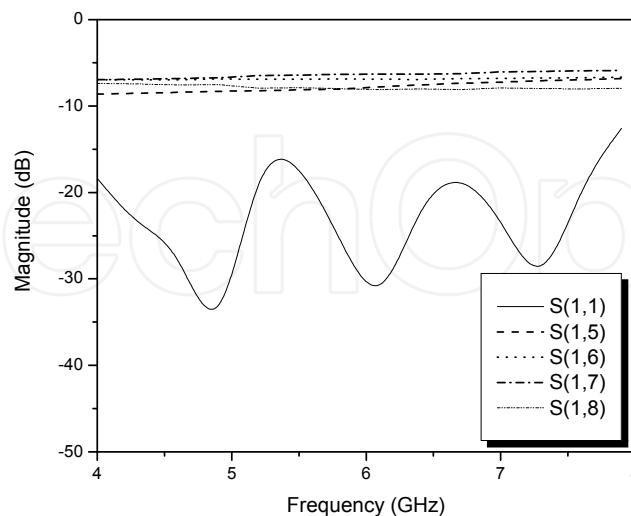
Fig. 29. Simulated results of multilayer Butler matrix.
