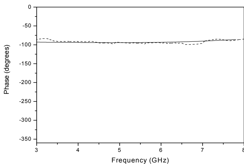
Fig. 20. Simulated and measured phase difference.
