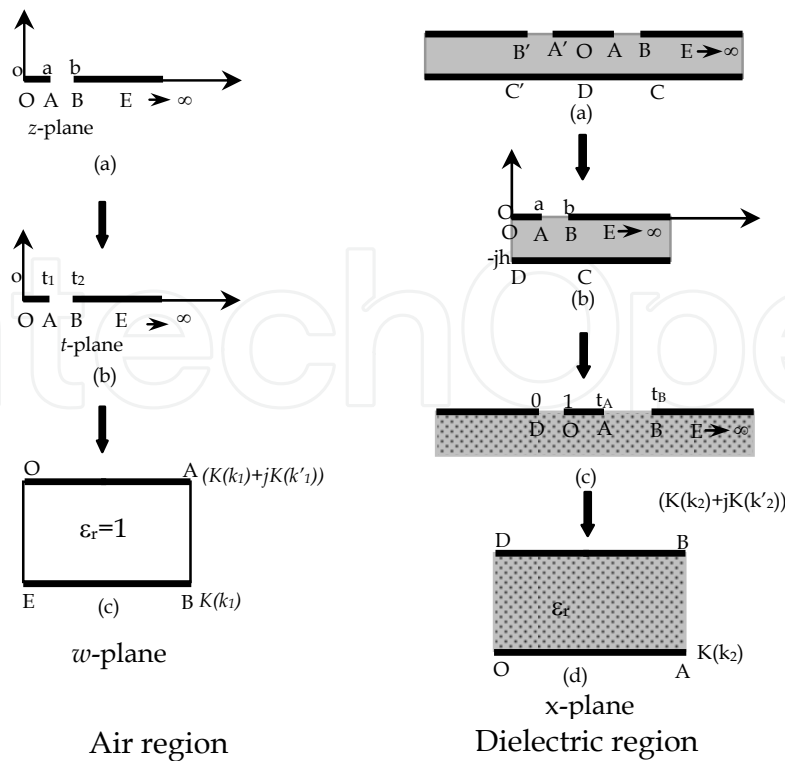
Fig. 13. Conformal mapping transformation of the odd-mode
