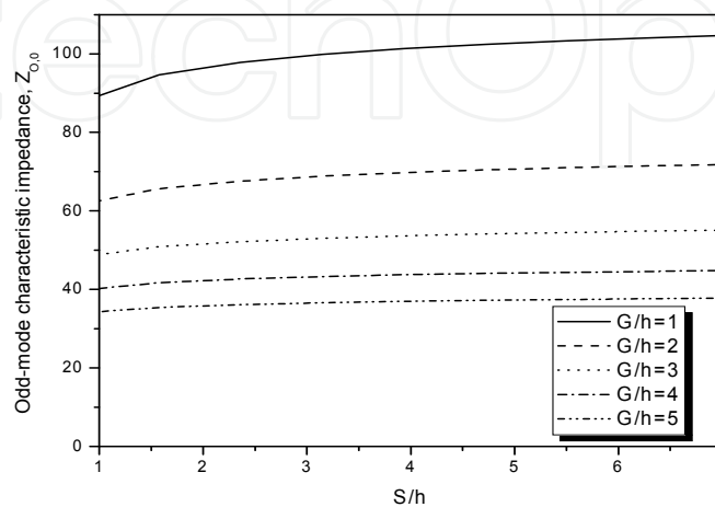
Fig. 15. Odd-mode characteristic impedance
