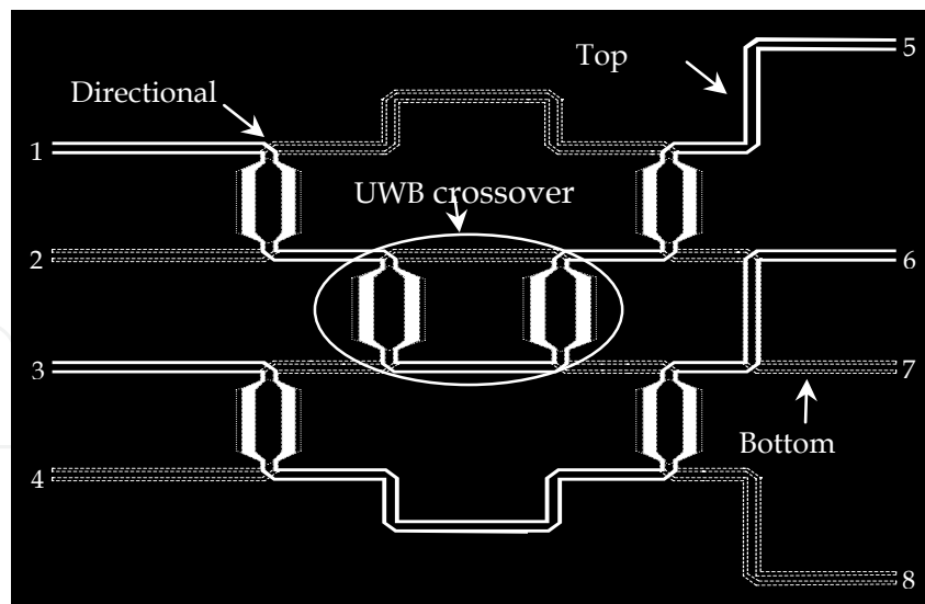
Fig. 28. Layout of UWB 4 X 4 Butler matrix
