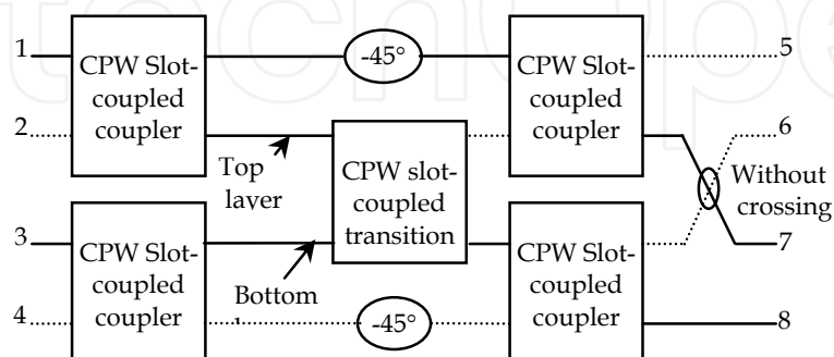
Fig. 27. Block diagram of the UWB Butler matrix.
