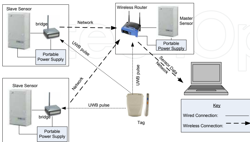
(a) Architecture of the portable UWB system
