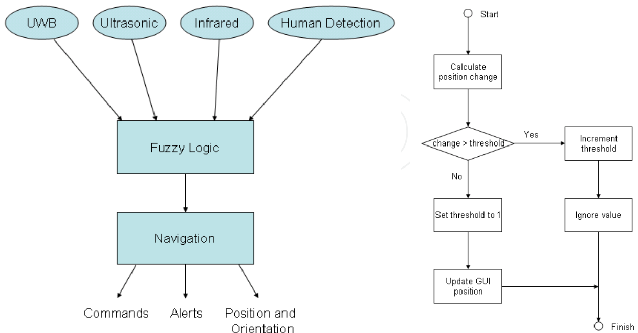
(b) Fuzzy logic flow chart
