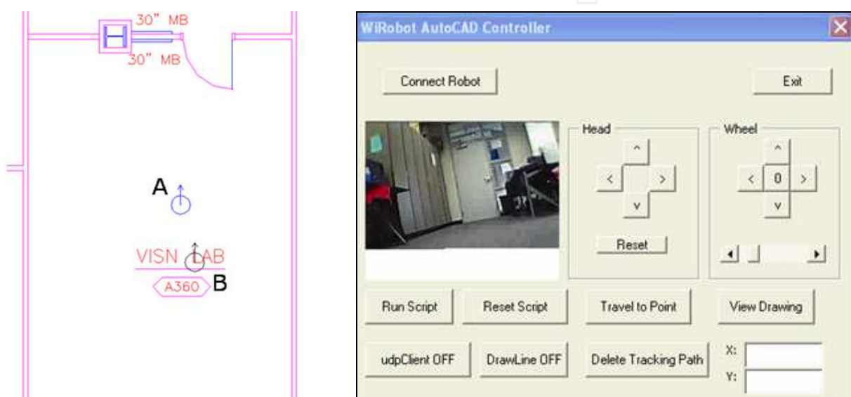
(a) Robot's dead reckoning position (A) and UWB position (B) (b) Real-time robot control GUI
