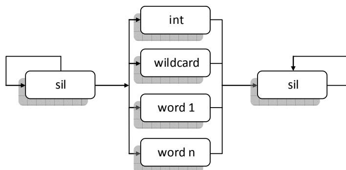
Fig. 4. Transition diagram of the AlfaNum Word Spotter
