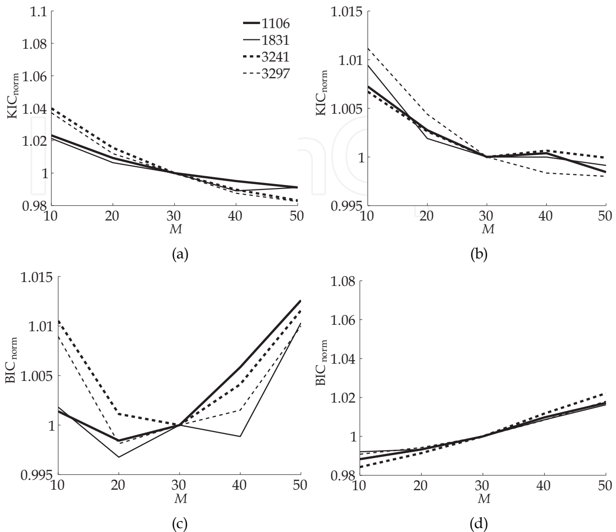
Fig. 3. KIC and BIC values as a function of GMM order (normalized with KIC and BIC values in case of 30 Gaussians), using clean and reverberant speech of male speakers. (a) KIC without reverberation, (b) KIC with RT=0.85 sec, (c) BIC without reverberation, and (d) BIC with RT=0.85 sec.
