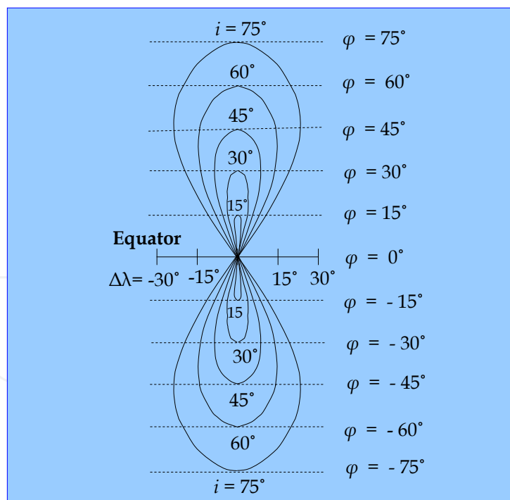
Fig. 38. Graphic illustration of why the spectator on the Earth sees relatively (apparent) motion of 24-hour satellites in circular orbit in relation to "still" Earth.
