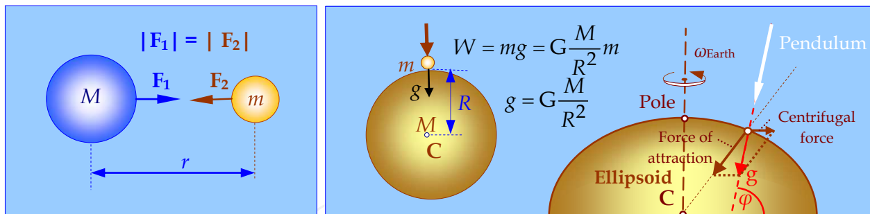
Fig. 15. Newton's Law of the universal gravitation.
