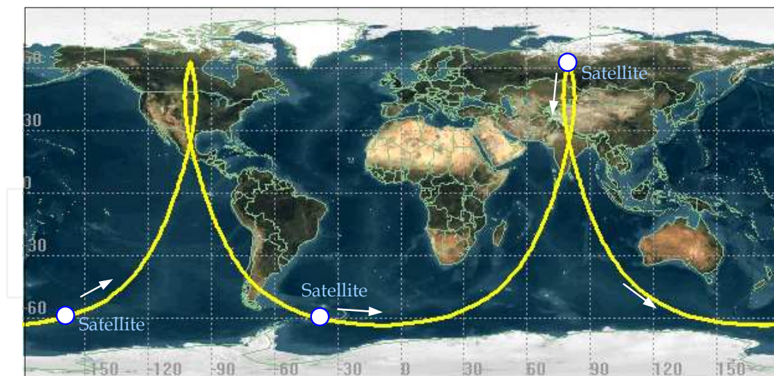
Fig. 44. Apparent trajectory of the satellites Molniya (URL 6).
