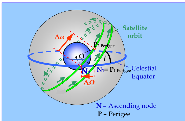
Fig. 30. Perturbations of the ascending node and perigee.
