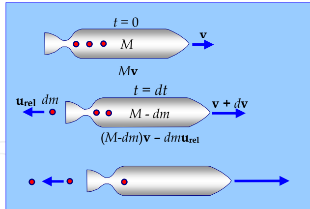
Fig. 7. The principle of a rocket operation.
