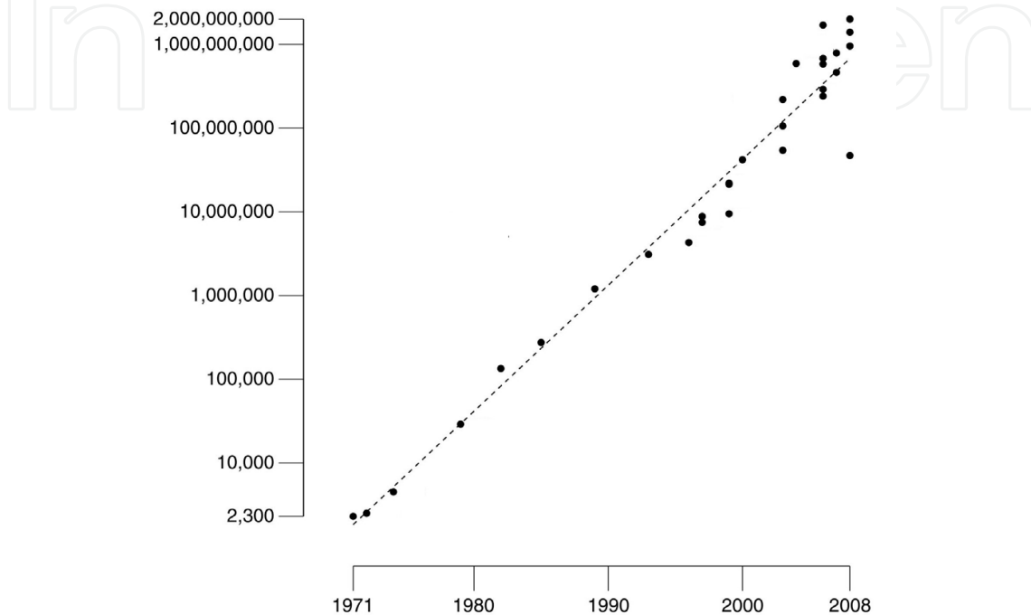
Fig. 1. One representation of the Moore-law. Horizontally the years, vertically the number of transistors in a CPU are represented. The points are for different CPU's between 1971 and 2008. The dashed line represents the Moore-law.
